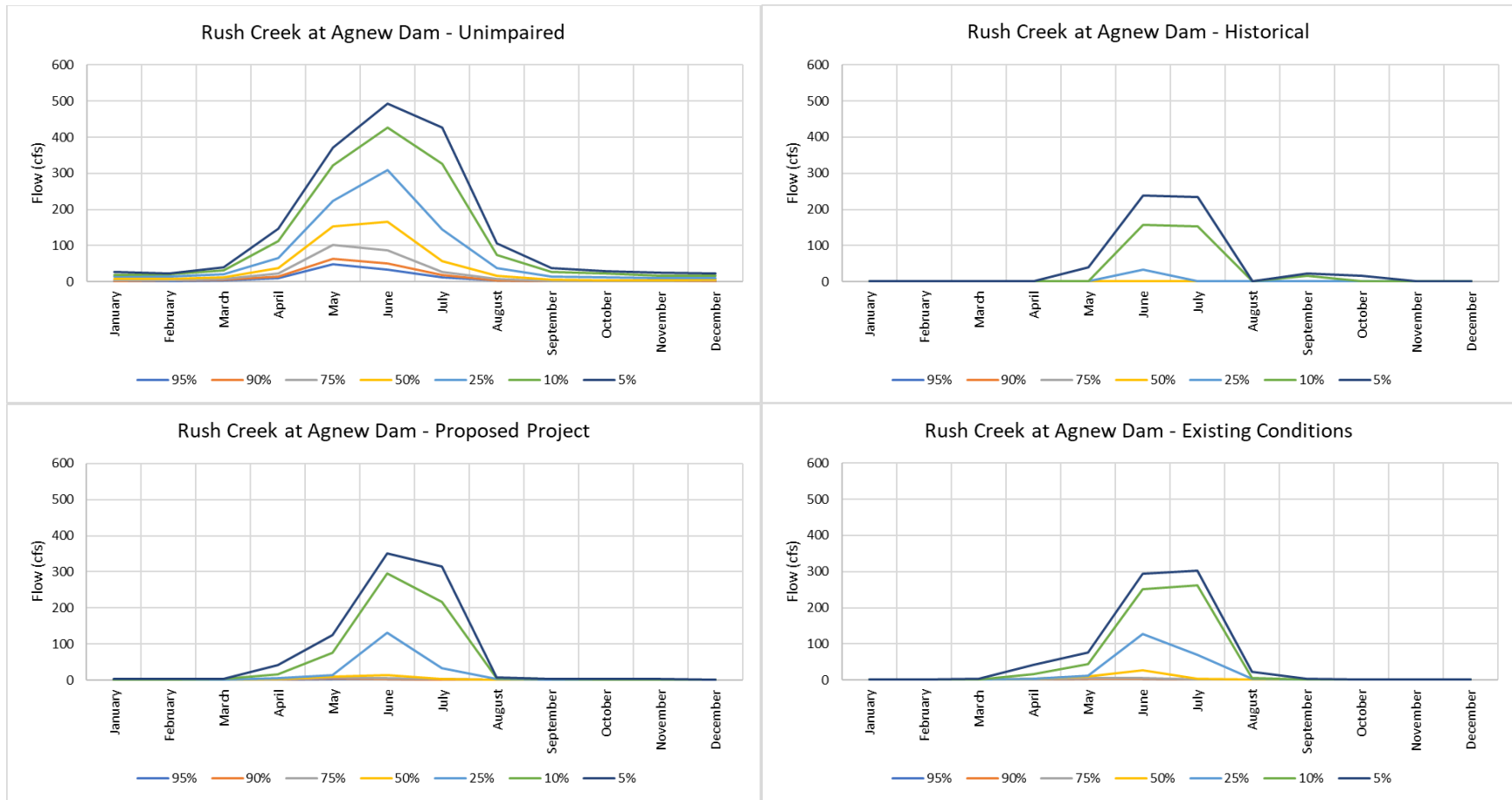
Figure AQ 2-49. January to December annual monthly flow exceedance plots 95%, 90%, 75%, 50% (median), 25%, 10%, and 5% exceedance for Rush Creek below Agnew Dam.
