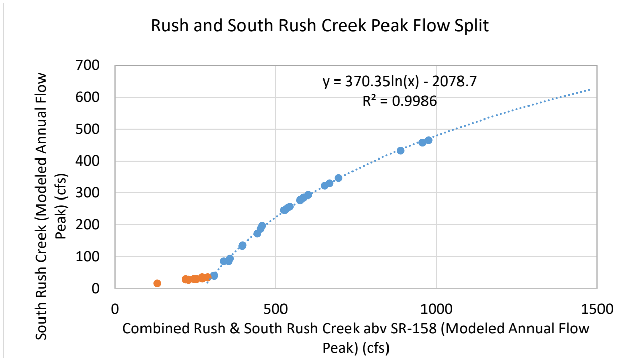
Figure AQ 2-75. Relationship between modeled peak annual flows at California State Route 158 for Rush Creek and South Rush Creek.
