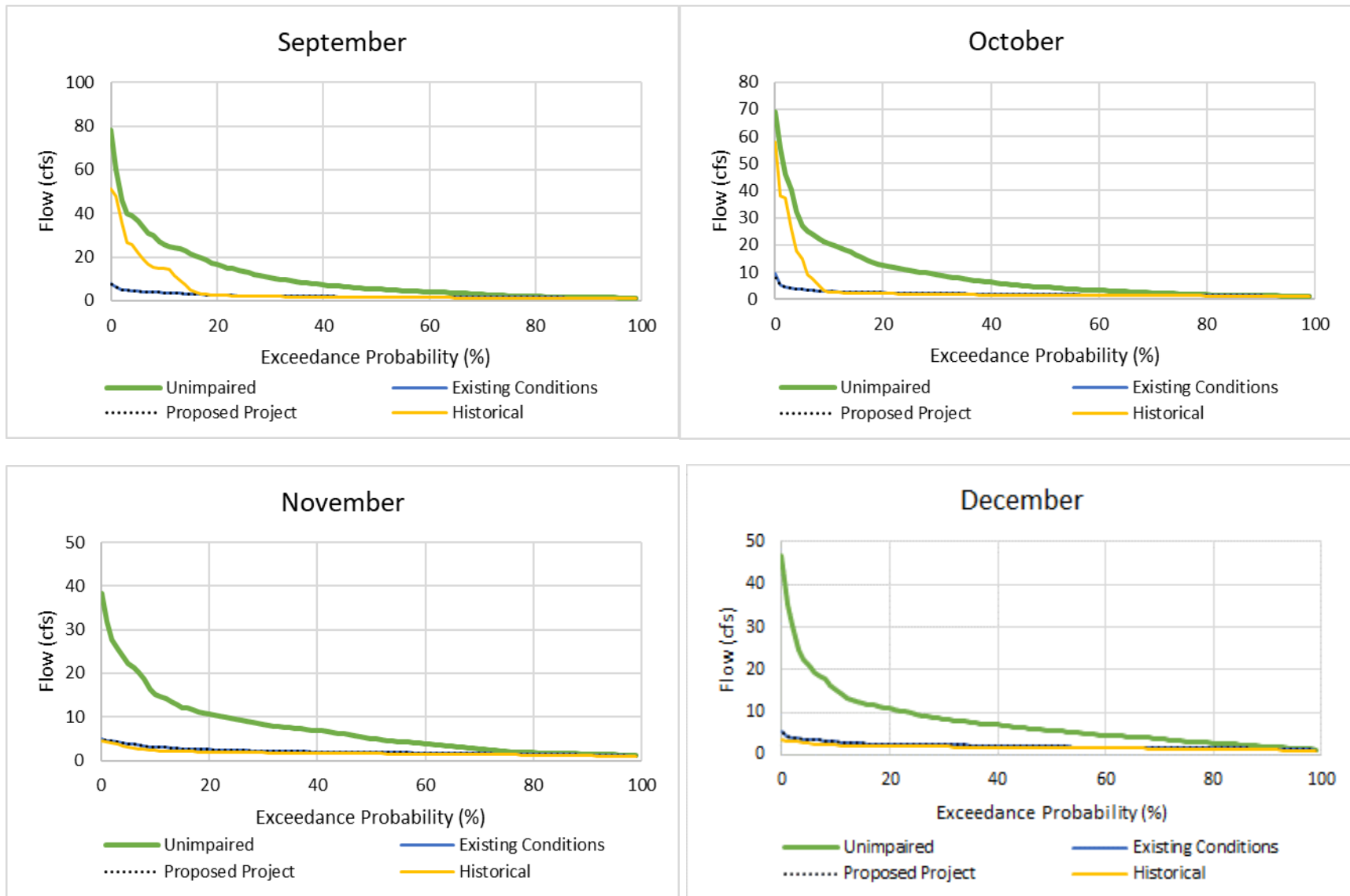
Figure AQ 2-37. Rush Creek above SR158 daily average flow exceedance by month (September-December).
