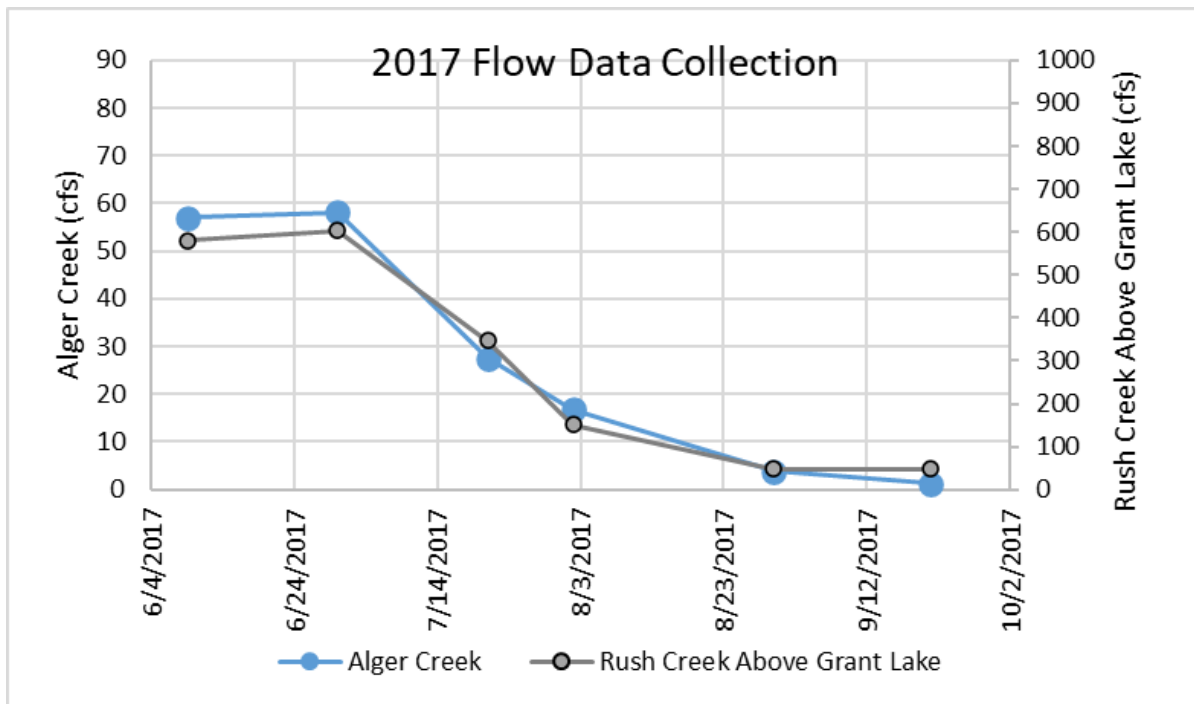
Figure AQ 2-74. Empirical flow data collected at Alger Creek in 2017 (left axis) compared to the Rush Creek above Grant Lake LADWP gage (right axis).
