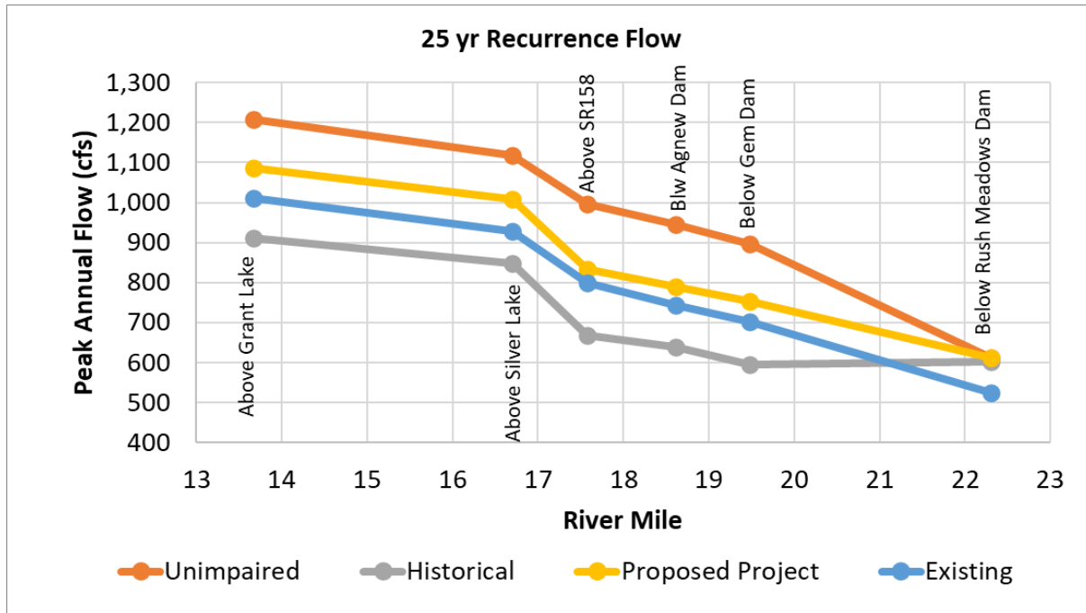
Figure AQ 2-70. Comparison of 25-year annual recurrence flow events for each of the scenarios (unimpaired, historical, Proposed Project, and existing) for different locations along Rush Creek (see labels).
