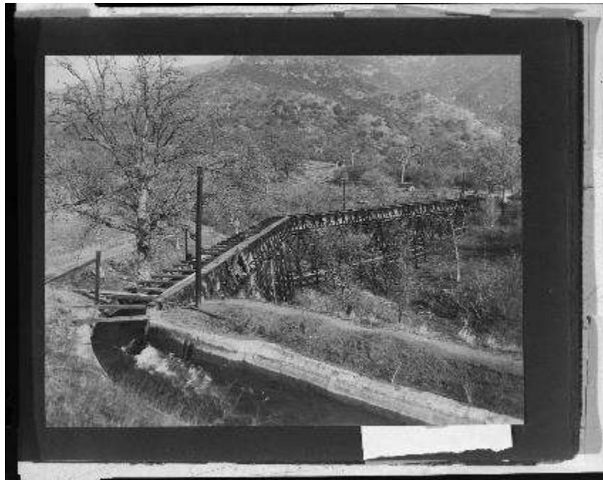
Figure 11: Kaweah No. 2 Concrete Ditch and Flume Section, circa 1908 (Huntington Digital Library, SCE Photograph Collection, Call Number 04 - 00732)
