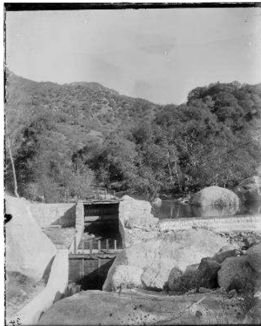
Figure 10: Kaweah No. 2 Diversion, 1908 (Huntington Digital Library, SCE Photograph Collection, Call Number 04 - 00034)
