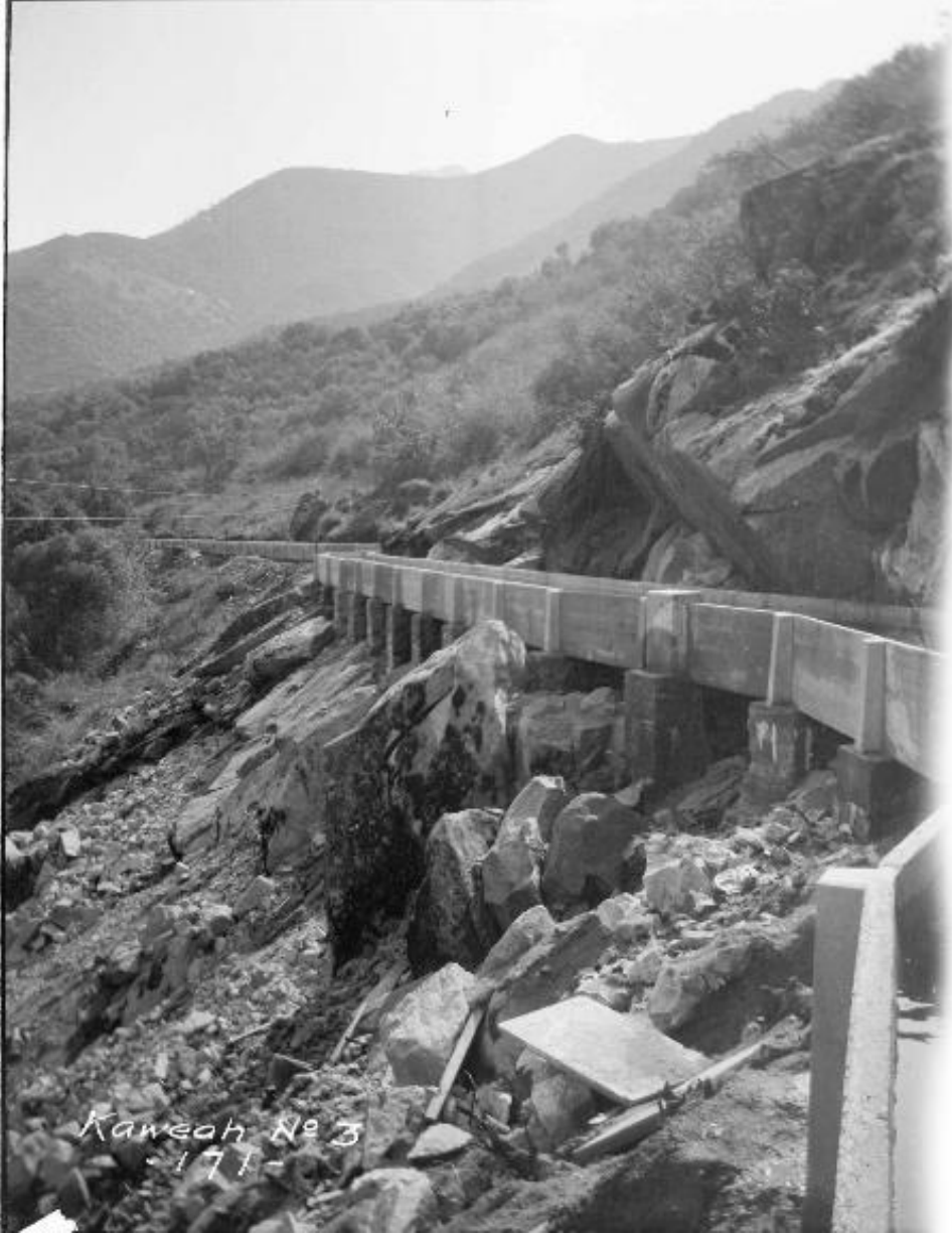
Figure CUL 5-22 Middle Fork Flowline, circa 1912
