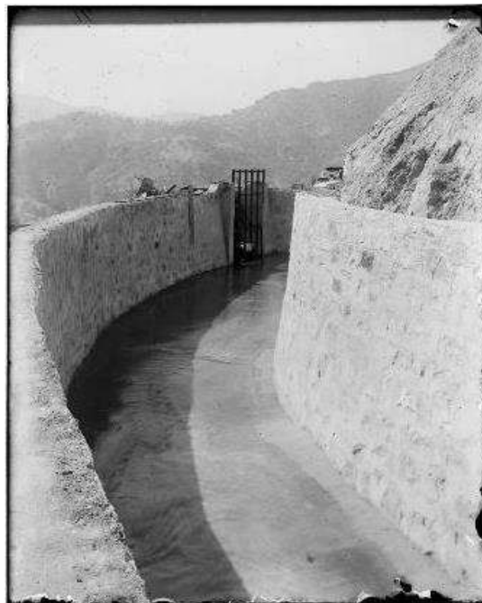
Figure 12: Kaweah No. 2 Forebay, 1908 (Huntington Digital Library, SCE Photograph Collection, Call Number 04 - 00071)
