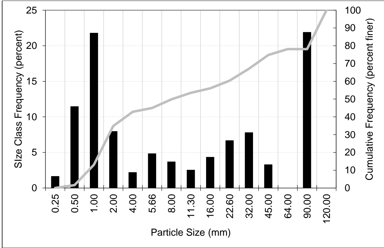
Figure A-11. Kaweah River Downstream of East Fork Kaweah Confluence and Upstream of Kaweah No. 1 Powerhouse: Histogram and Cumulative Particle Size Distribution, Sample 2 Subsample 1
