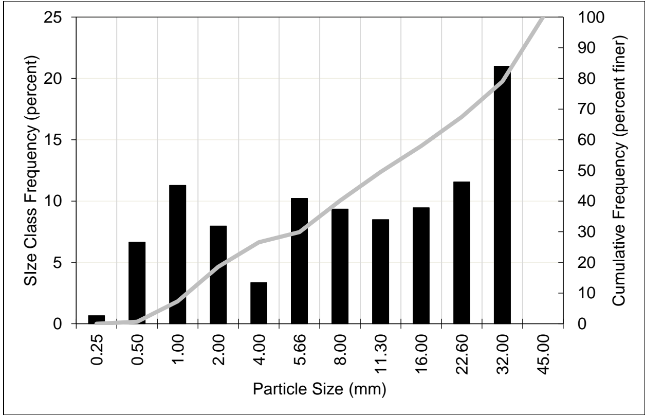
Figure A-16. Kaweah River Downstream of Kaweah No. 2 Powerhouse: Histogram and Cumulative Particle Size Distribution, Sample 2 Subsample 2
