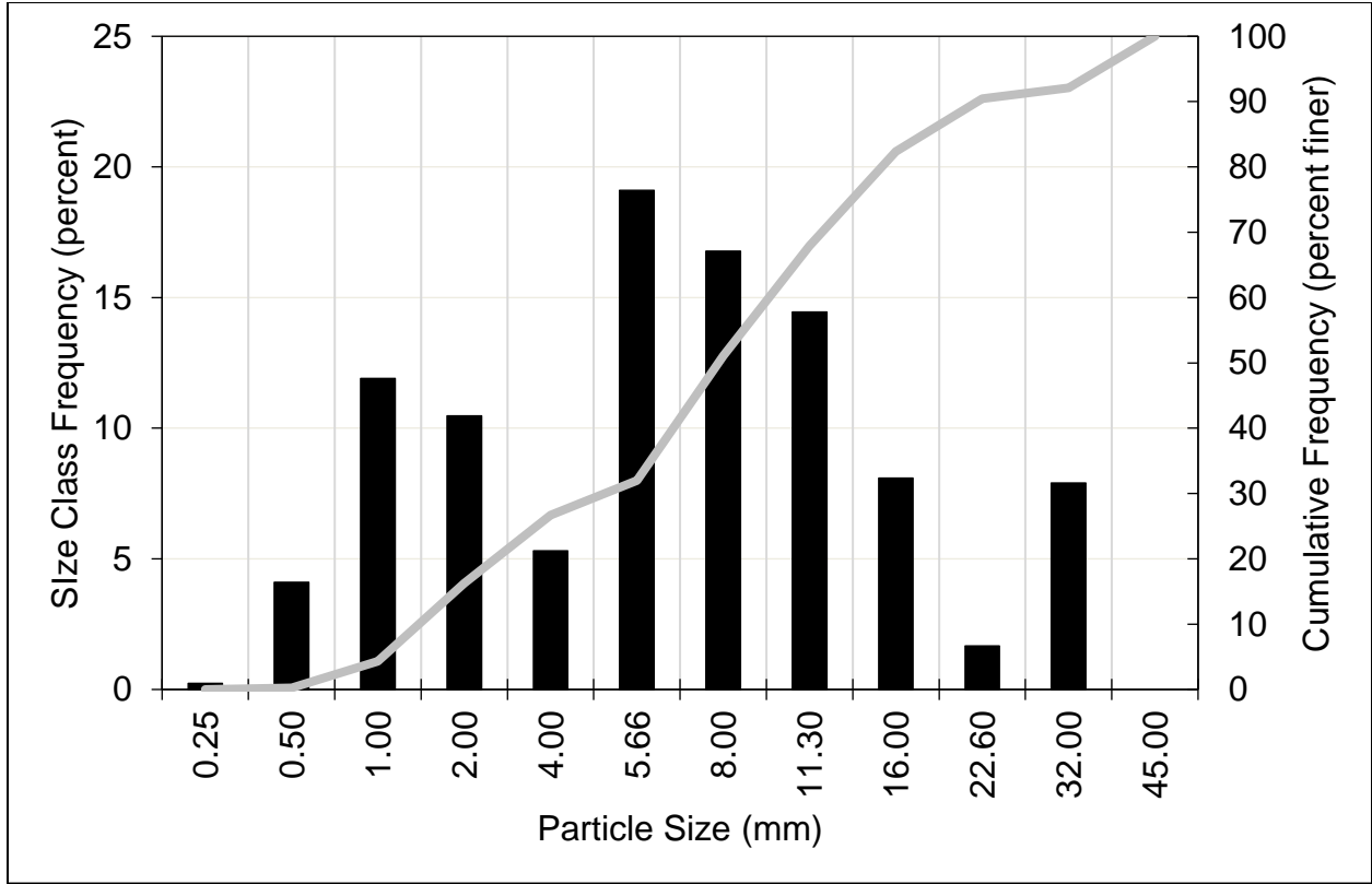
Figure A-22. East Fork Kaweah River Downstream of the Kaweah No. 1 Diversion: Histogram and Cumulative Particle Size Distribution, Sample 1 Subsample 2
