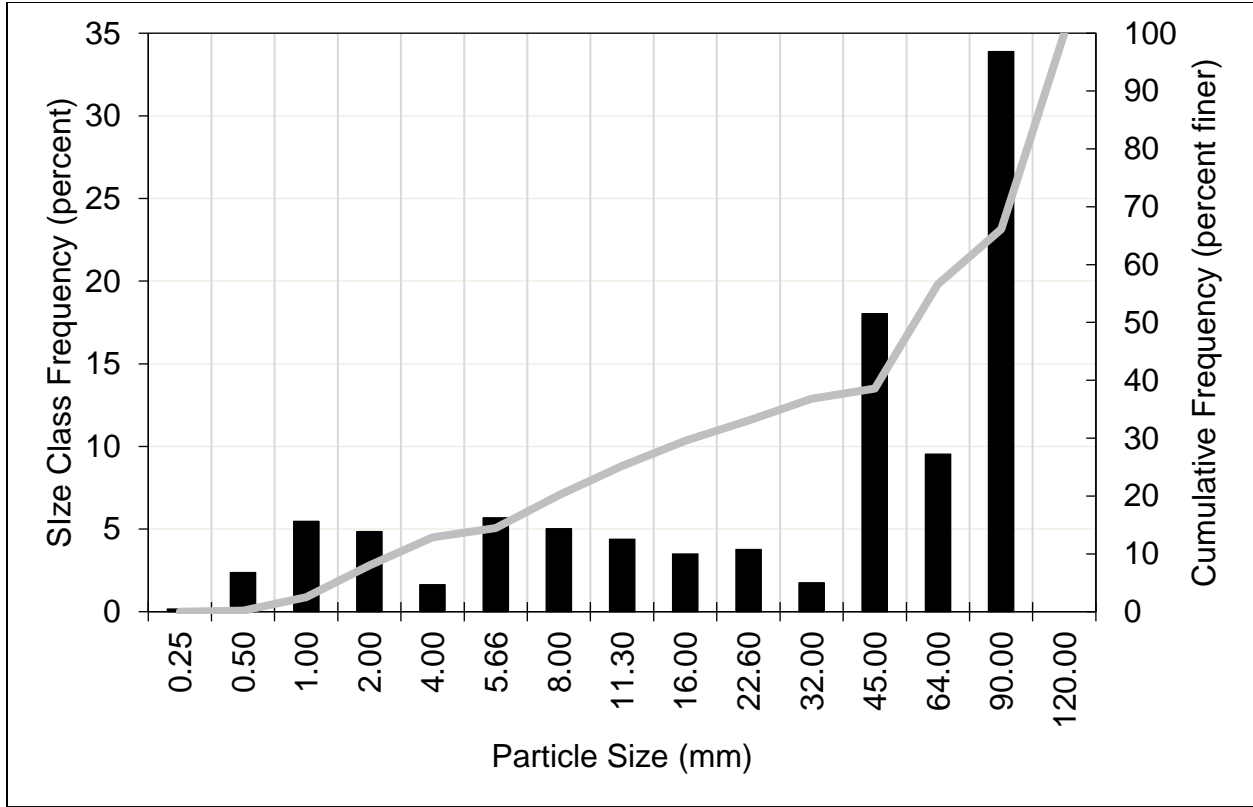
Figure A-20. East Fork Kaweah River Upstream of the Kaweah No. 1 Diversion: Histogram and Cumulative Particle Size Distribution, Sample 2 Subsample 2
