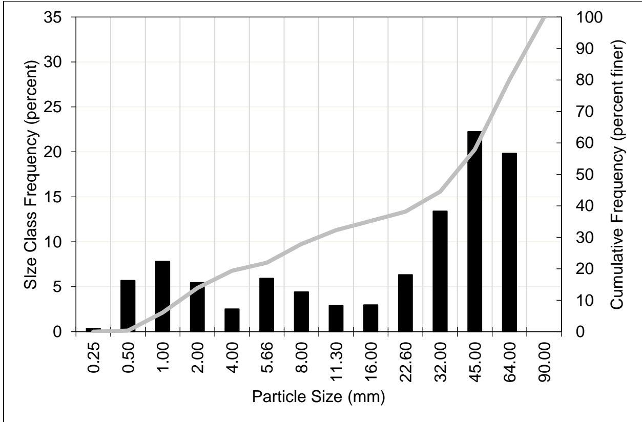
Figure A-5. Kaweah River Downstream of Kaweah No. 3 Powerhouse and Upstream of the East Fork Kaweah River Confluence Spawning Gravel: Histogram and Cumulative Particle Size Distribution, Sample 1 Subsample 1
