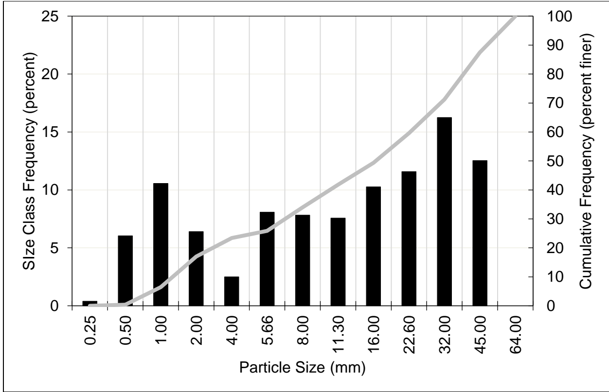
Figure A-3. Kaweah River Upstream of Kaweah No. 3 Powerhouse Spawning Gravel: Histogram and Cumulative Particle Size Distribution, Sample 2 Subsample 1
