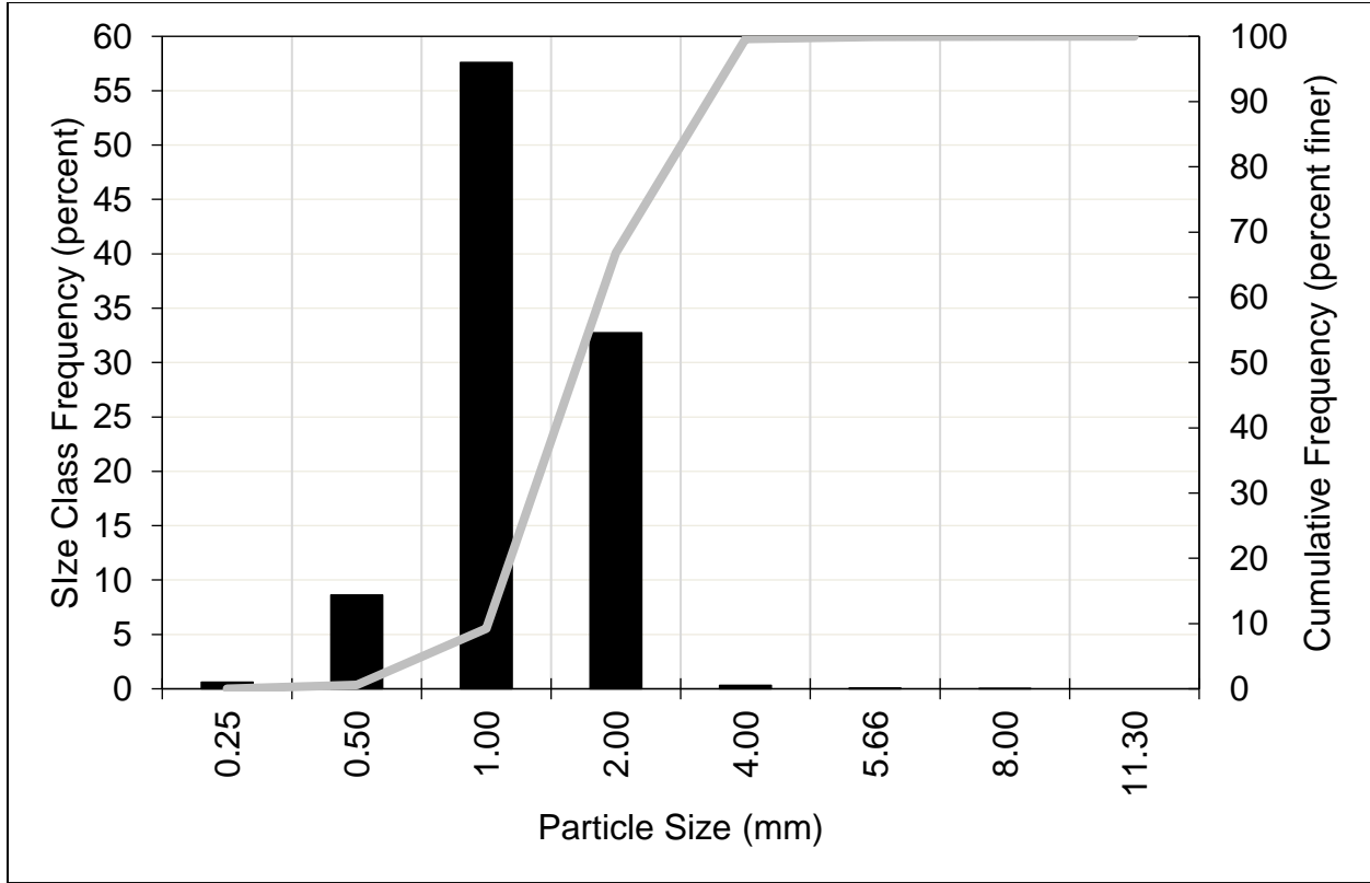
Figure A-27. East Fork Kaweah River Upstream of Confluence with Kaweah River: Histogram and Cumulative Particle Size Distribution, Sample 2 Subsample 1
