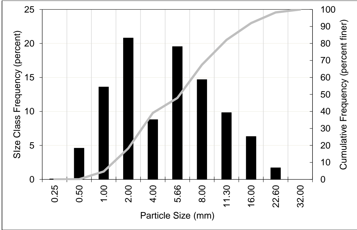
Figure A-25. East Fork Kaweah River Upstream of Confluence with Kaweah River: Histogram and Cumulative Particle Size Distribution, Sample 1 Subsample 1
