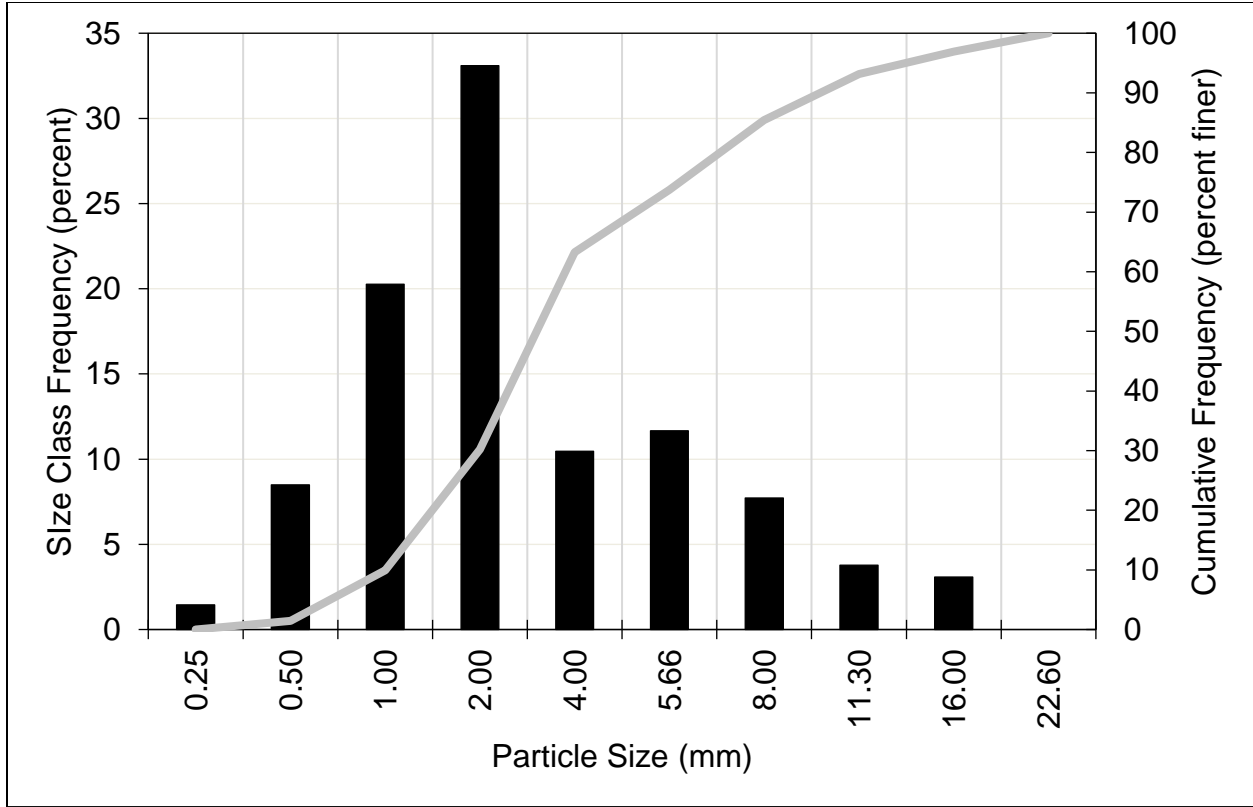
Figure A-26. East Fork Kaweah River Upstream of Confluence with Kaweah River: Histogram and Cumulative Particle Size Distribution, Sample 1 Subsample 2
