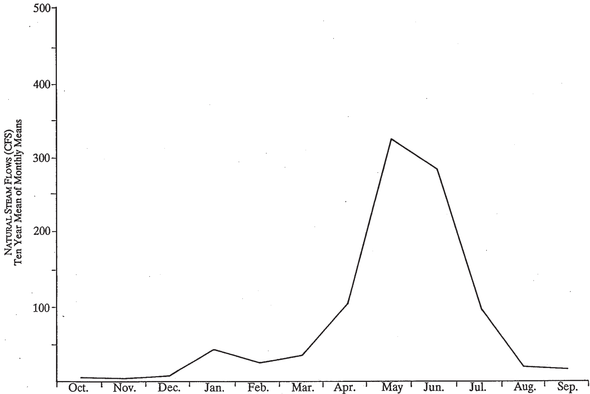
MARBLE FORK KAWEAH NO. 3 INTAKE - TEN YEAR MEAN OF MONTHLY MEAN FLOWS
