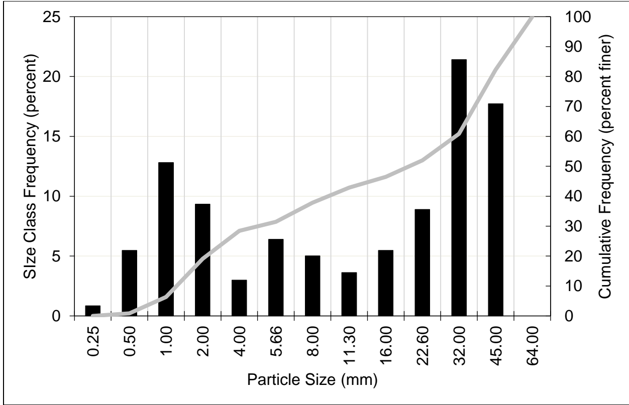
Figure A-9. Kaweah River Downstream of East Fork Kaweah Confluence and Upstream of Kaweah No. 1 Powerhouse: Histogram and Cumulative Particle Size Distribution, Sample 1 Subsample 1
