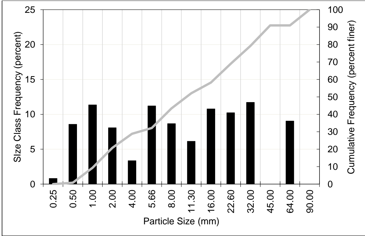
Figure A-7. Kaweah River Downstream of Kaweah No. 3 Powerhouse and Upstream of the East Fork Kaweah River Confluence Spawning Gravel: Histogram and Cumulative Particle Size Distribution, Sample 2 Subsample 1
