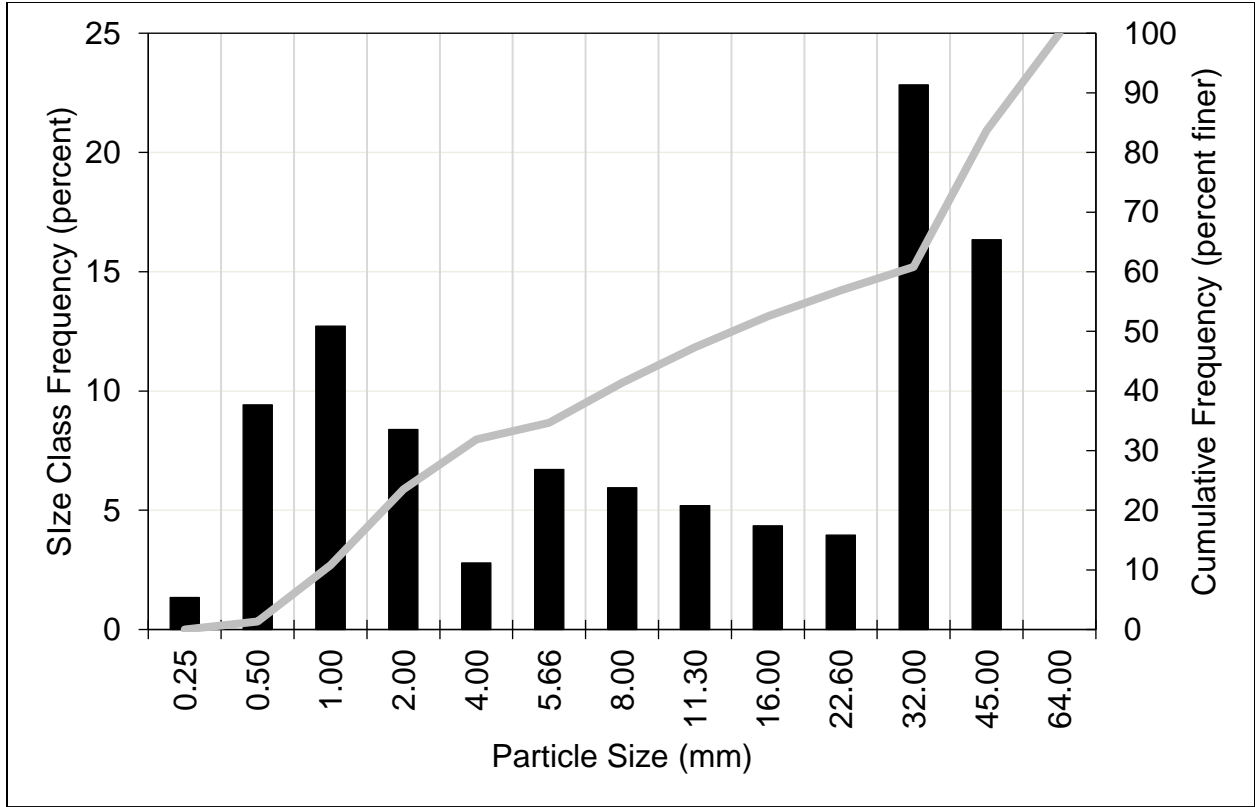
Figure A-12. Kaweah River Downstream of East Fork Kaweah Confluence and Upstream of Kaweah No. 1 Powerhouse: Histogram and Cumulative Particle Size Distribution, Sample 2 Subsample 2
