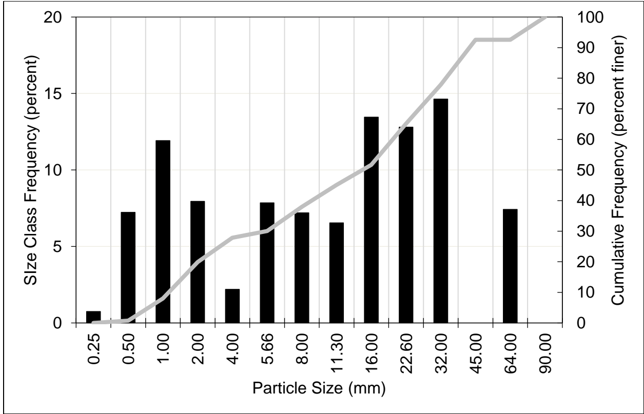
Figure A-14. Kaweah River Downstream of Kaweah No. 2 Powerhouse: Histogram and Cumulative Particle Size Distribution, Sample 1 Subsample 2
