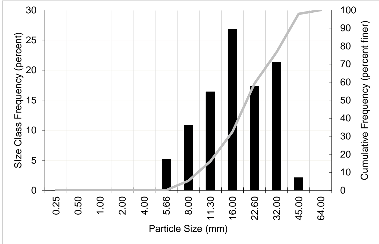
Figure A-23. East Fork Kaweah River Downstream of the Kaweah No. 1 Diversion: Histogram and Cumulative Particle Size Distribution, Sample 2 Subsample 1
