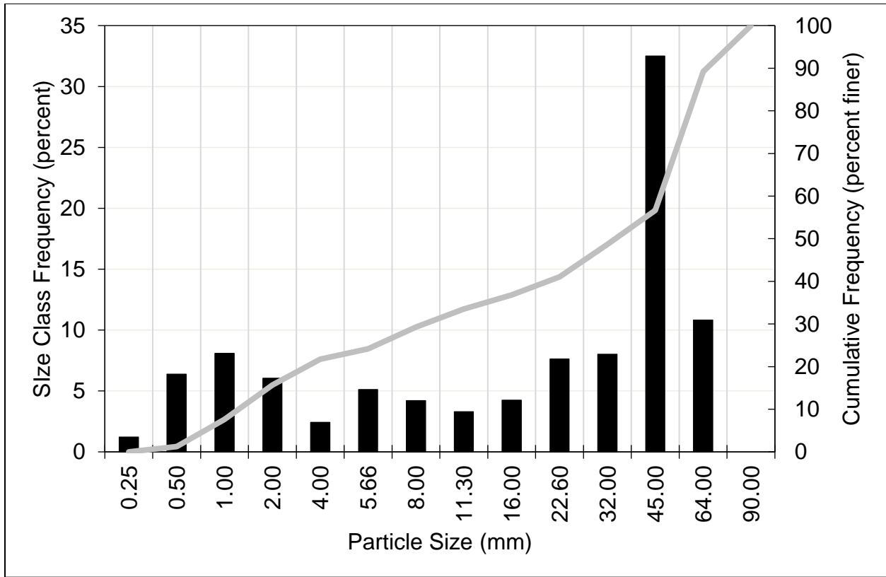
Figure A-6. Kaweah River Downstream of Kaweah No. 3 Powerhouse and Upstream of the East Fork Kaweah River Confluence Spawning Gravel: Histogram and Cumulative Particle Size Distribution, Sample 1 Subsample 2
