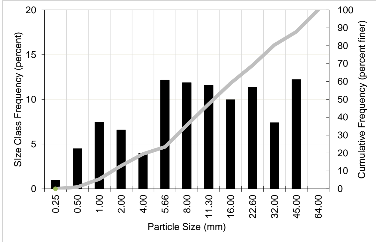
Figure A-19. East Fork Kaweah River Upstream of the Kaweah No. 1 Diversion: Histogram and Cumulative Particle Size Distribution, Sample 2 Subsample 1
