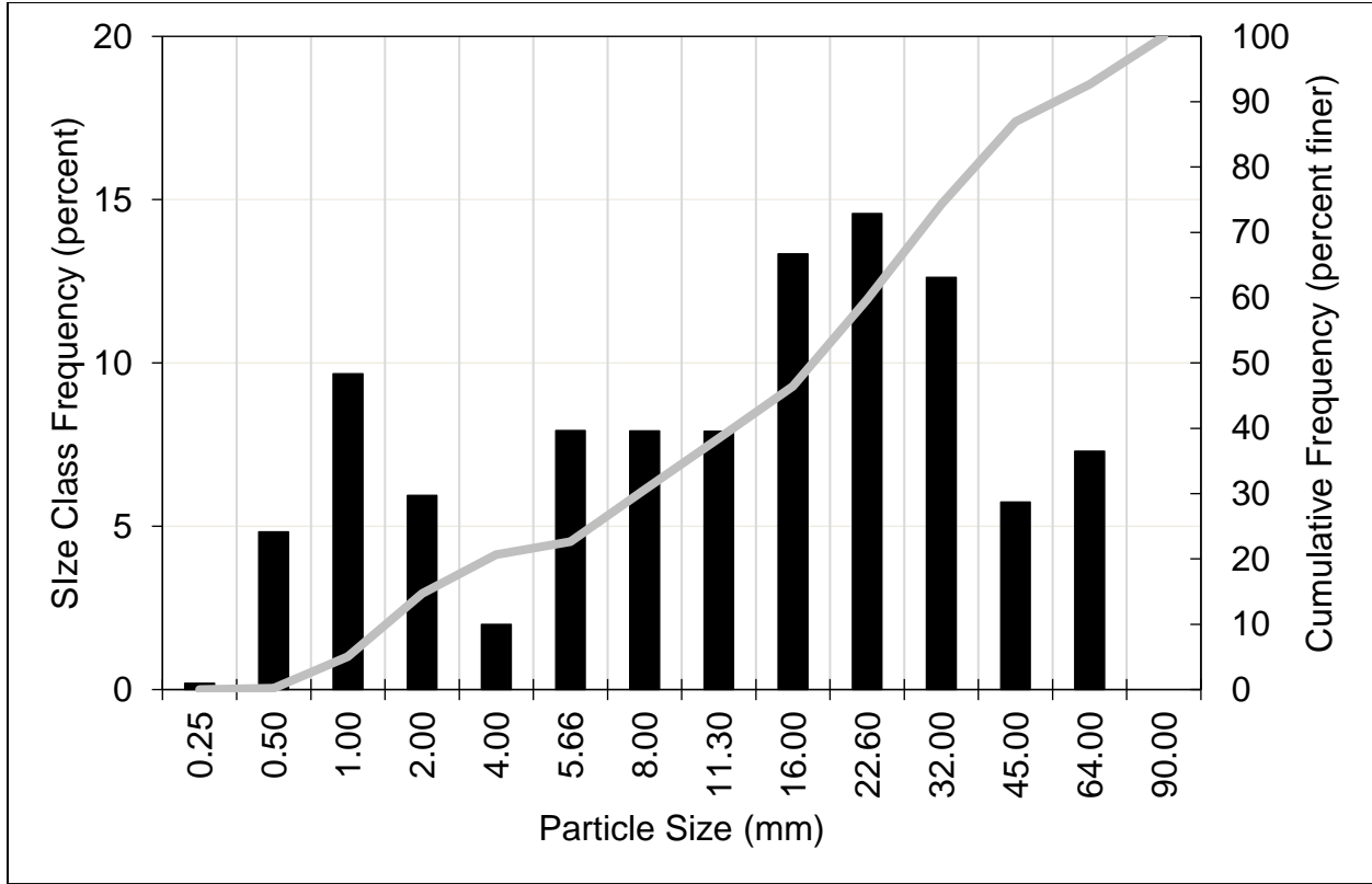
Figure A-13. Kaweah River Downstream of Kaweah No. 2 Powerhouse: Histogram and Cumulative Particle Size Distribution, Sample 1 Subsample 1
