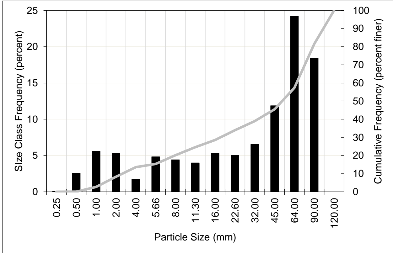
Figure A-17. East Fork Kaweah River Upstream of the Kaweah No. 1 Diversion: Histogram and Cumulative Particle Size Distribution, Sample 1 Subsample 1
