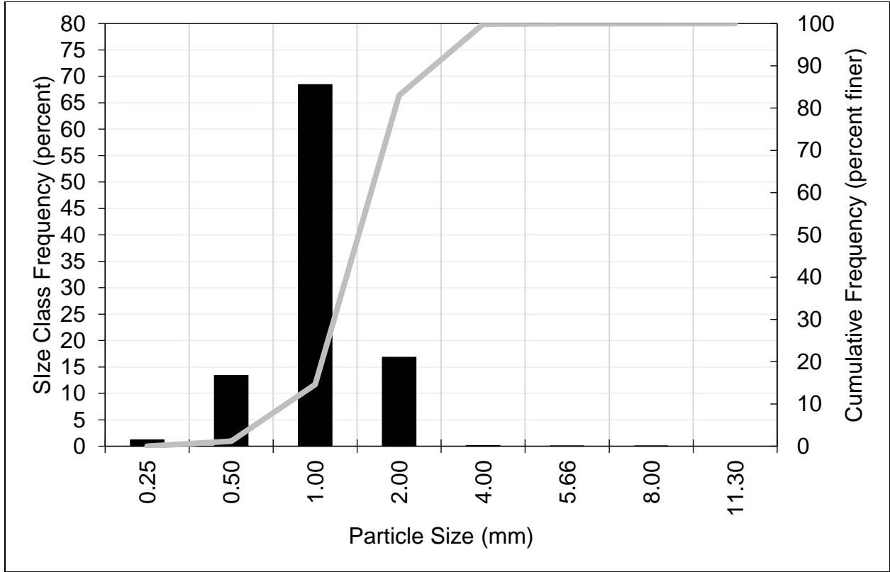
Figure A-28. East Fork Kaweah River Upstream of Confluence with Kaweah River: Histogram and Cumulative Particle Size Distribution, Sample 2 Subsample 2
