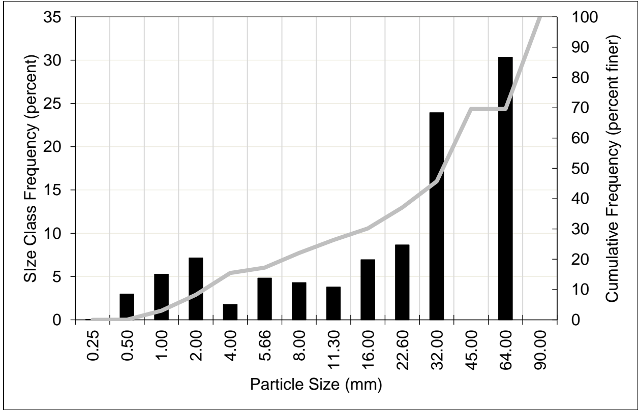
Figure A-18. East Fork Kaweah River Upstream of the Kaweah No. 1 Diversion: Histogram and Cumulative Particle Size Distribution, Sample 1 Subsample 2
