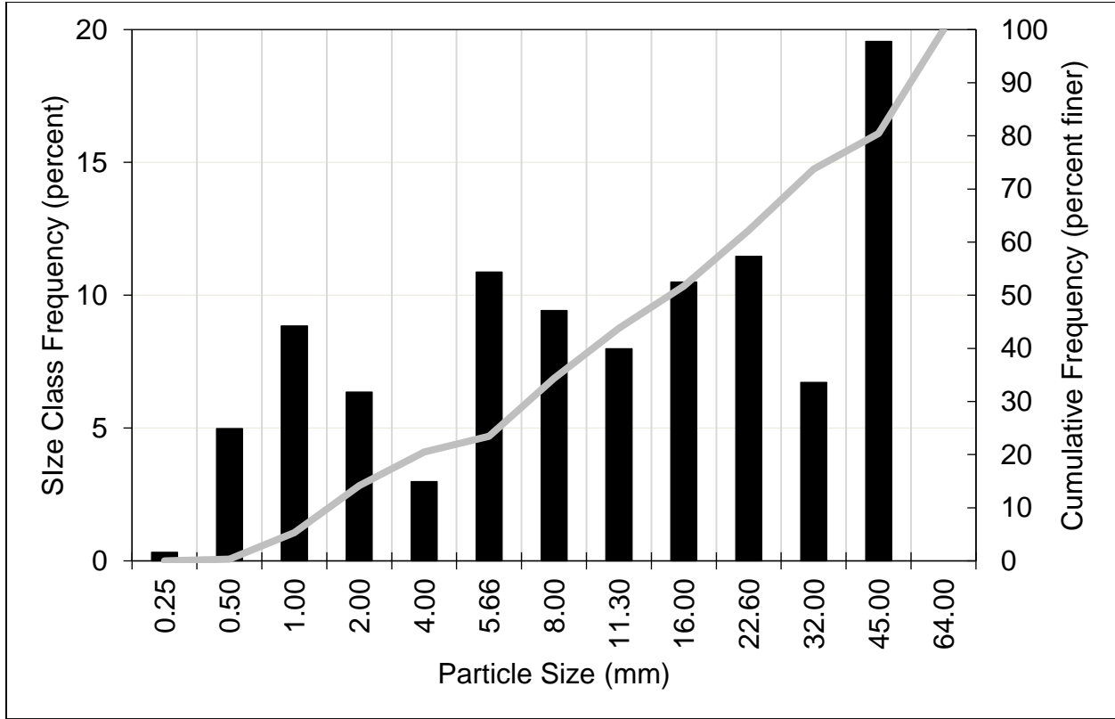
Figure A-15. Kaweah River Downstream of Kaweah No. 2 Powerhouse: Histogram and Cumulative Particle Size Distribution, Sample 2 Subsample 1
