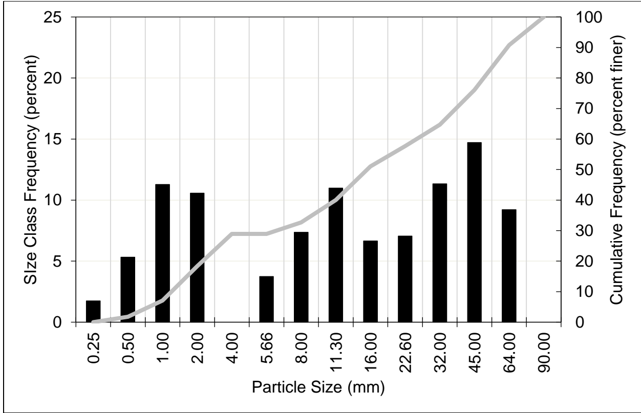
Figure A-1. Kaweah River Upstream of Kaweah No. 3 Powerhouse Spawning Gravel: Histogram and Cumulative Particle Size Distribution, Sample 1 Subsample 1
