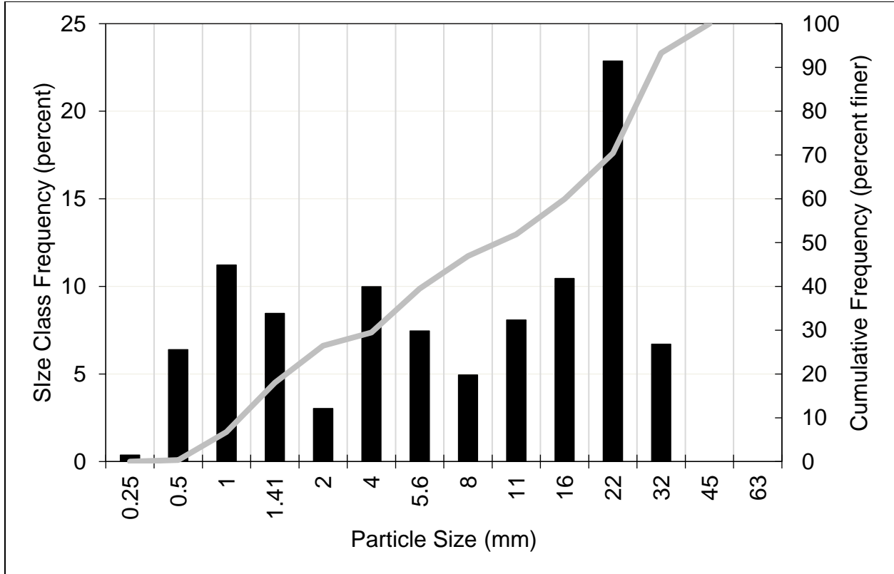
Figure A-8. Kaweah River Downstream of Kaweah No. 3 Powerhouse and Upstream of the East Fork Kaweah River Confluence Spawning Gravel: Histogram and Cumulative Particle Size Distribution, Sample 2 Subsample 2
