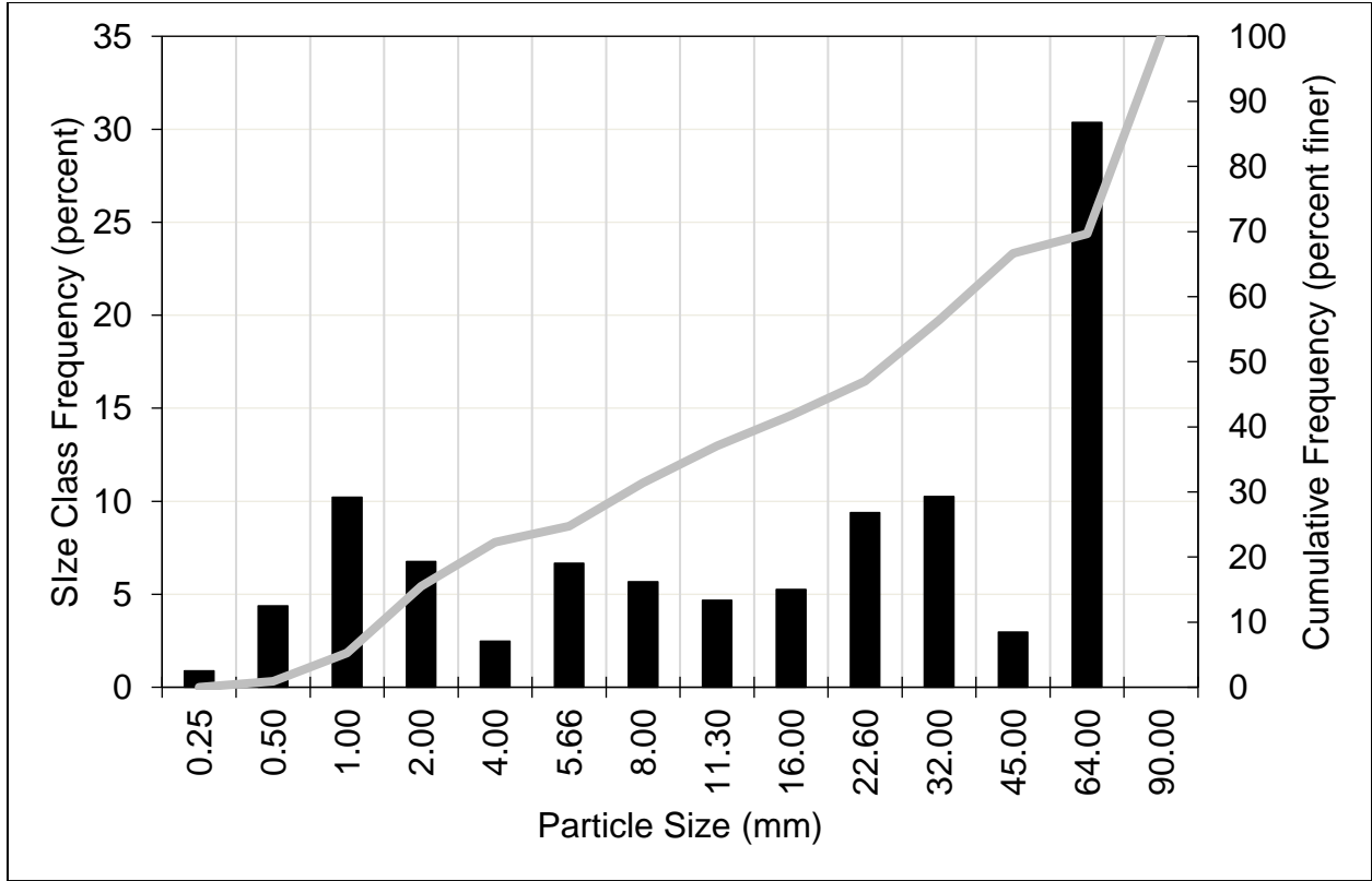
Figure A-2. Kaweah River Upstream of Kaweah No. 3 Powerhouse Spawning Gravel: Histogram and Cumulative Particle Size Distribution, Sample 1 Subsample 2
