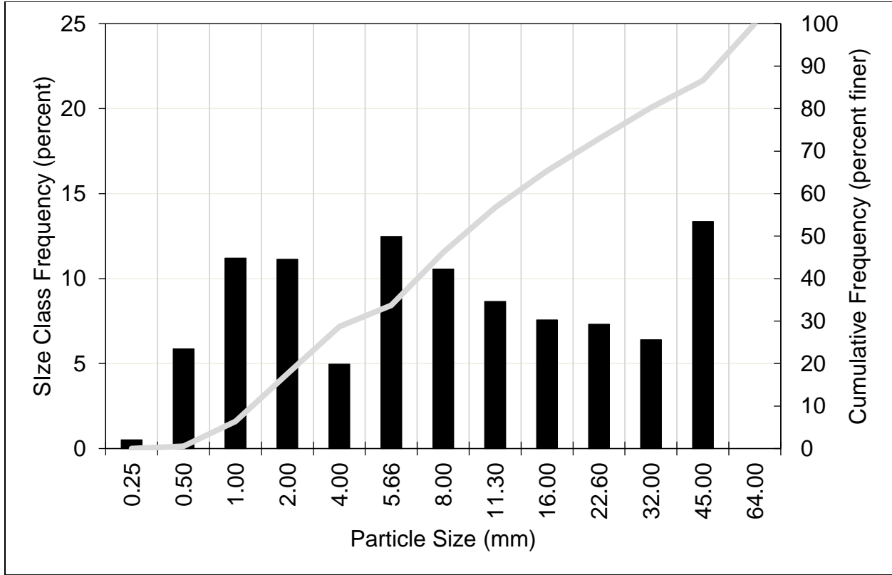
Figure A-21. East Fork Kaweah River Downstream of the Kaweah No. 1 Diversion: Histogram and Cumulative Particle Size Distribution, Sample 1 Subsample 1
