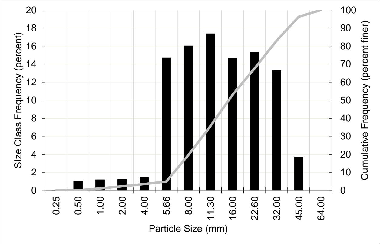
Figure A-24. East Fork Kaweah River Downstream of the Kaweah No. 1 Diversion: Histogram and Cumulative Particle Size Distribution, Sample 2 Subsample 2
