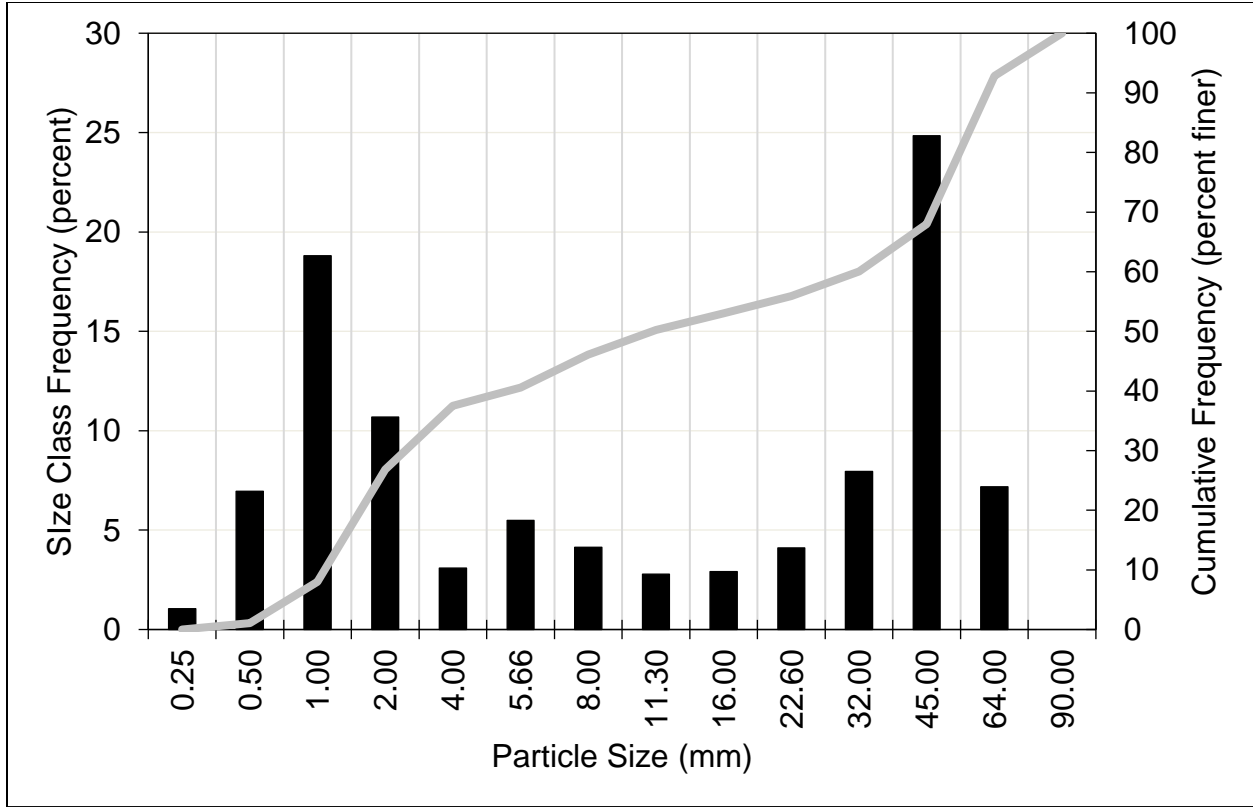
Figure A-10. Kaweah River Downstream of East Fork Kaweah Confluence and Upstream of Kaweah No. 1 Powerhouse: Histogram and Cumulative Particle Size Distribution, Sample 1 Subsample 2
