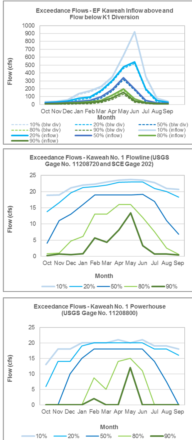
Figure B-3a. Monthly Exceedance Flows (10%, 20%, 50%, 80%, and 90%) in the East Fork Kaweah River Bypass Reach and Kaweah No. 1 Flowline, and at the Kaweah No. 1 Powerhouse (WY 1994–2018) 4
