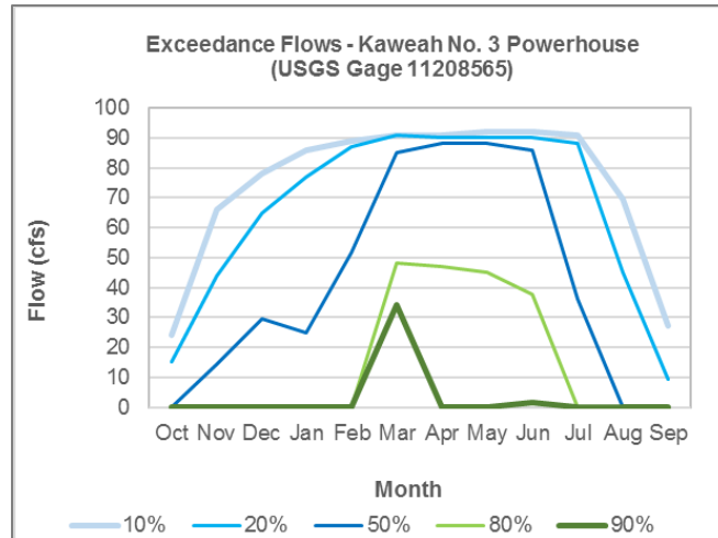
Figure B-3c. Monthly Exceedance Flows (10%, 20%, 50%, 80%, and 90%) at the Kaweah No. 3 Powerhouse (WY 2002–2018) 6
