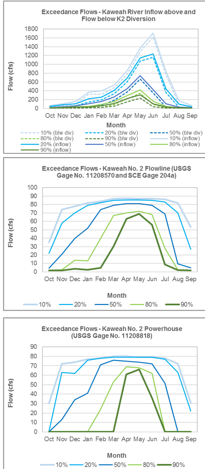
Figure B-3b. Monthly Exceedance Flows (10%, 20%, 50%, 80%, and 90%) in the Kaweah River Bypass Reach and Kaweah No. 2 Flowline, and at the Kaweah No. 2 Powerhouse (WY 1994–2018) 5
