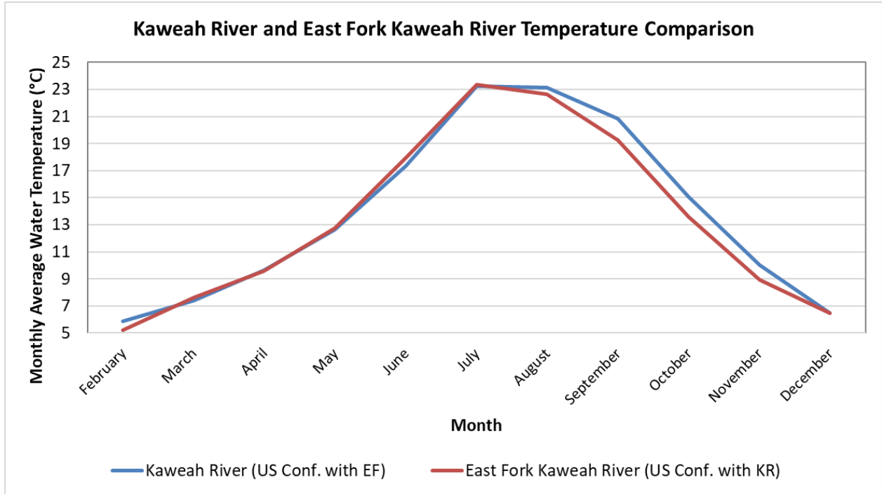
Figure AQ 4-14. Comparison of Monthly Average Water Temperatures on the Kaweah River Upstream of Conf. with the East Fork and the East Fork River Upstream of the Conf. with the Kaweah River.
