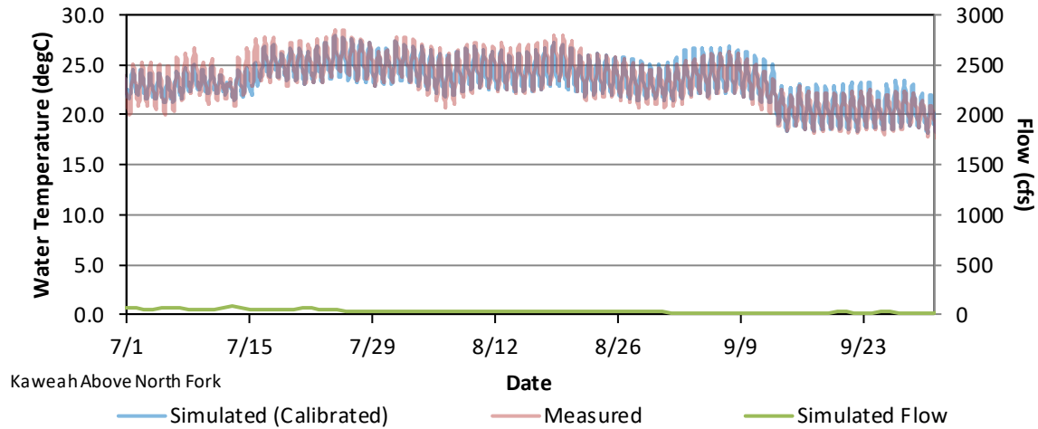
Figure E- 19. Water Temperature Model Calibration Results for Kaweah River Downstream of Powerhouse #2 for July 1 – September 30, 2018.
