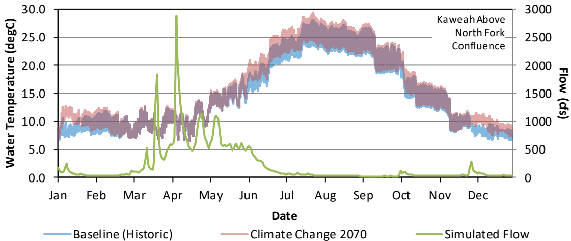
Figure AQ 4-11. Hourly Water Temperature and Daily Average Flow Model Results for the Baseline (Existing) and Climate Change 2070 for Kaweah River Upstream of the Confluence with the North Fork, January 1 – December 31, 2018.
