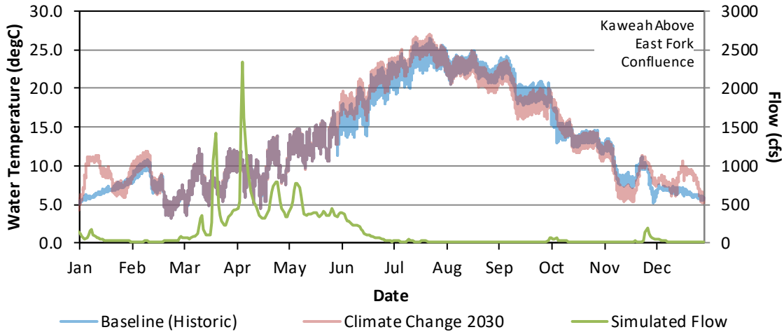
Figure G - 66. Hourly Water Temperature and Daily Average Flow Model Results for the Baseline (Historic) and Climate Change 2030 for Kaweah River Upstream of the Confluence with the East Fork, January 1 – December 31, 2018.
