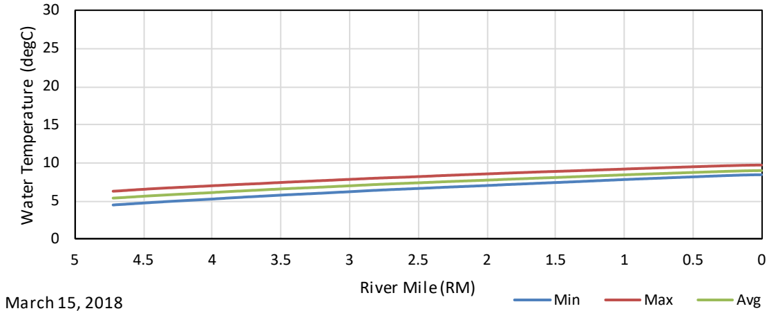
Figure G - 106. March 15, 2018 Baseline (Historic) Maximum, Average, and Minimum Longitudinal Water Temperature Profiles in the East Fork of the Kaweah River Upstream of the Confluence with the Mainstem.
