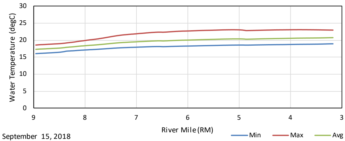
Figure G - 59. September 15, 2018 Climate Change 2030 Maximum, Average, and Minimum Longitudinal Water Temperature Profiles in the Kaweah River Upstream of Powerhouse #2.
