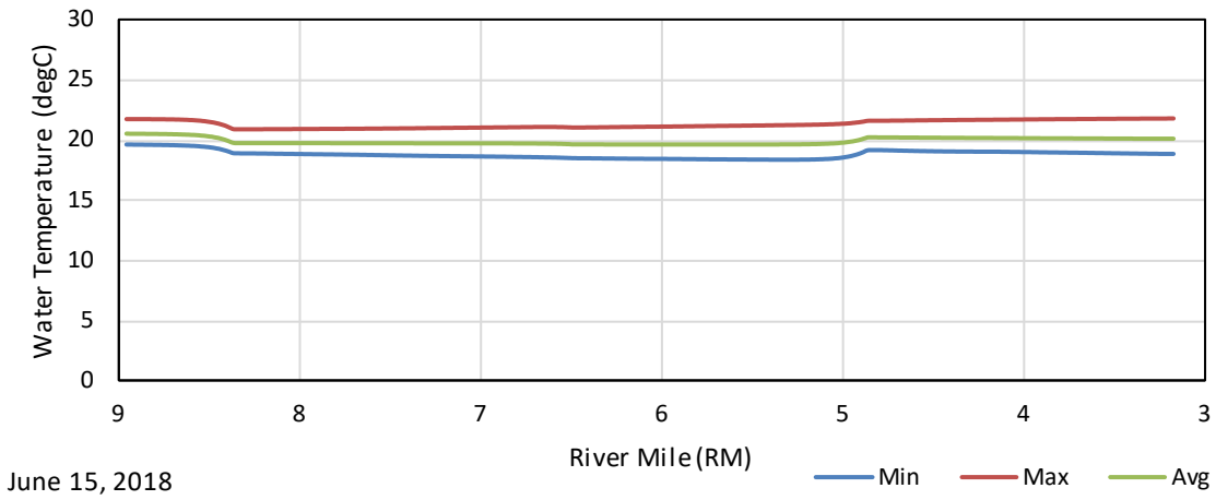
Figure G - 56. June 15, 2018 Climate Change 2070 Maximum, Average, and Minimum Longitudinal Water Temperature Profiles in the Kaweah River Upstream of Powerhouse #1.
