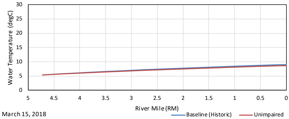
Figure F - 35. March 15, 2018 Average Longitudinal Water Temperature Profile in the East Fork of the Kaweah River Upstream of the Confluence with the Kaweah River for the Baseline (Historic) and Unimpaired Simulations.
