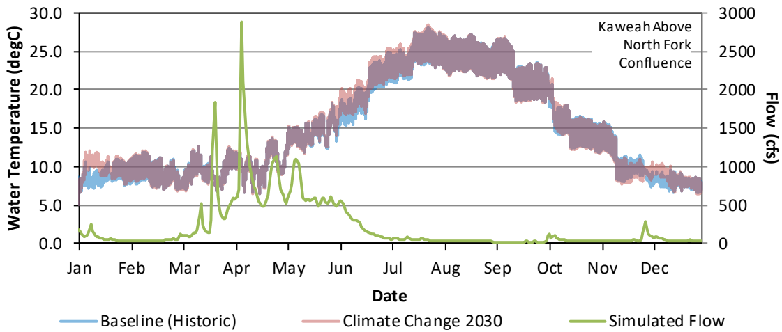
Figure G - 81. Hourly Water Temperature and Daily Average Flow Model Results for the Baseline (Historic) and Climate Change 2030 for Kaweah River Upstream of the Confluence with the North Fork, January 1 – December 31, 2018.
