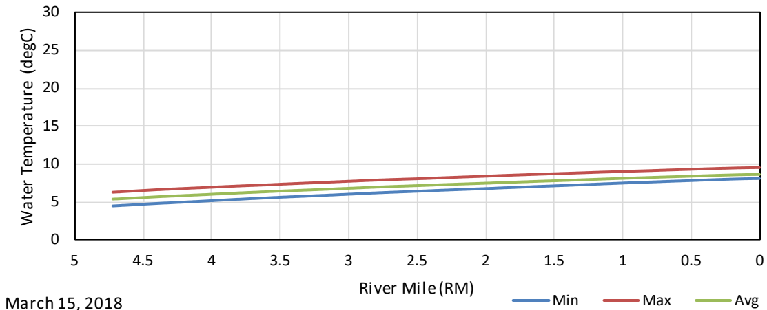
Figure F - 34. March 15, 2018 Unimpaired Maximum, Average, and Minimum Longitudinal Water Temperature Profiles in the East Fork of the Kaweah River Upstream of the Confluence with the Kaweah River.
