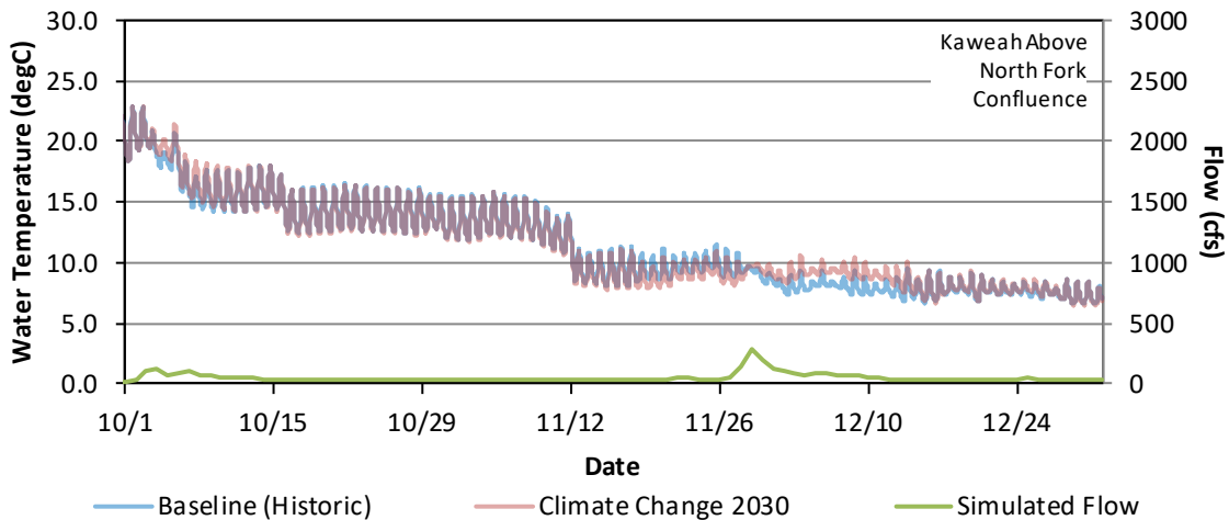
Figure G - 85. Hourly Water Temperature and Daily Average Flow Model Results for the Baseline (Historic) and Climate Change 2030 for Kaweah River Upstream of the Confluence with the North Fork, October 1 – December 31, 2018.
