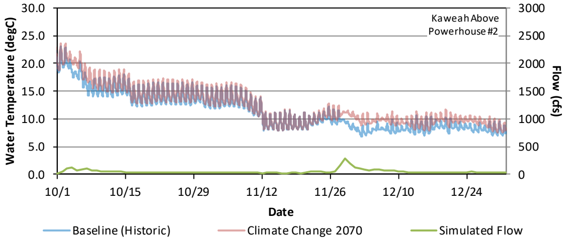
Figure G - 100. Hourly Water Temperature and Daily Average Flow Model Results for the Baseline (Historic) and Climate Change 2070 for Kaweah River Upstream of Powerhouse #2, October 1 – December 31, 2018.
