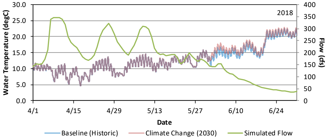
Figure G - 124. Hourly Water Temperature Model Results Baseline (Historic) and Climate Change 2030 for East Fork of the Kaweah River Upstream of the Confluence with the Kaweah River for April 1 – June 30, 2018.
