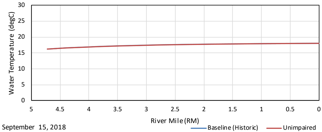
Figure F - 41. September 15, 2018 Average Longitudinal Water Temperature Profile in the East Fork of the Kaweah River Upstream of the Confluence with the Kaweah River for the Baseline (Historic) and Unimpaired Simulations.
