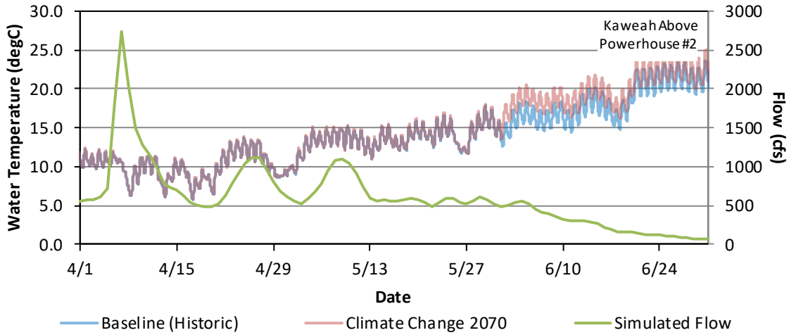
Figure G - 98. Hourly Water Temperature and Daily Average Flow Model Results for the Baseline (Historic) and Climate Change 2070 for Kaweah River Upstream of Powerhouse #2, April 1 – June 30, 2018.
