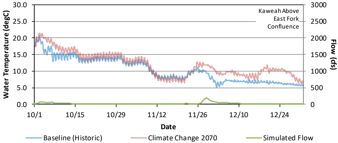
Figure G - 90. Hourly Water Temperature and Daily Average Flow Model Results for the Baseline (Historic) and Climate Change 2070 for Kaweah River Upstream of the Confluence with the East Fork, October 1 – December 31, 2018.
