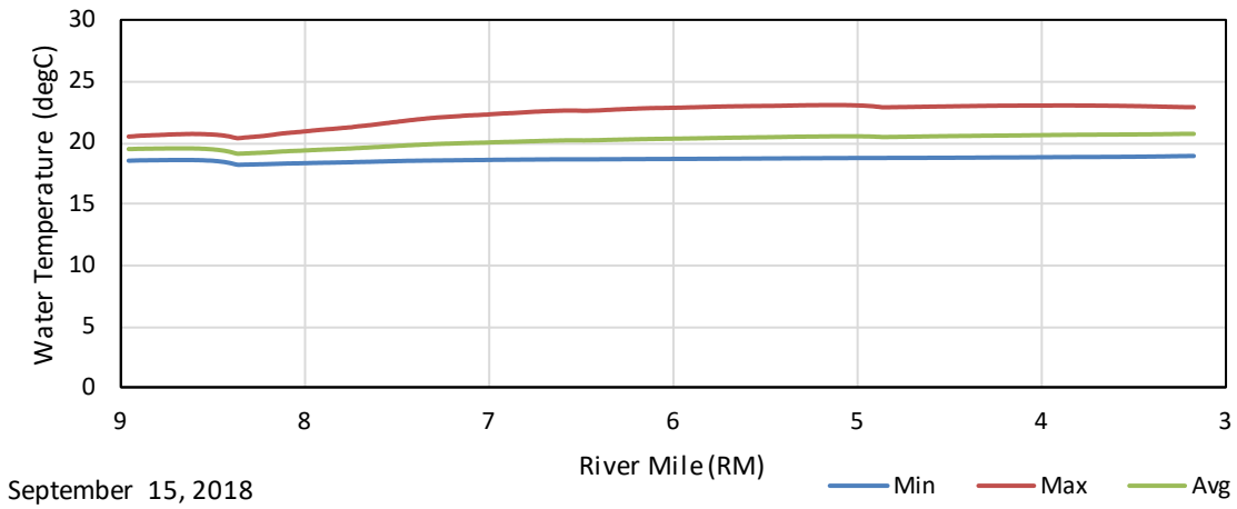
Figure G - 58. September 15, 2018 Baseline (Historic) Maximum, Average, and Minimum Longitudinal Water Temperature Profiles in the Kaweah River Upstream of Powerhouse #2.
