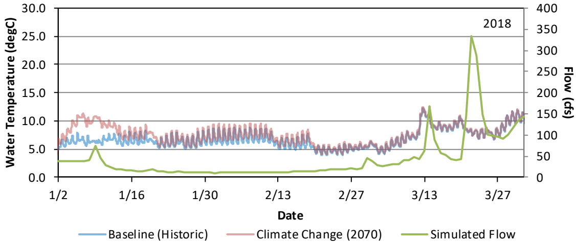
Figure G - 128. Hourly Water Temperature Model Results Baseline (Historic) and Climate Change 2070 East Fork of the Kaweah River Upstream of the Confluence with the Kaweah River for January 1 – March 31, 2018.
