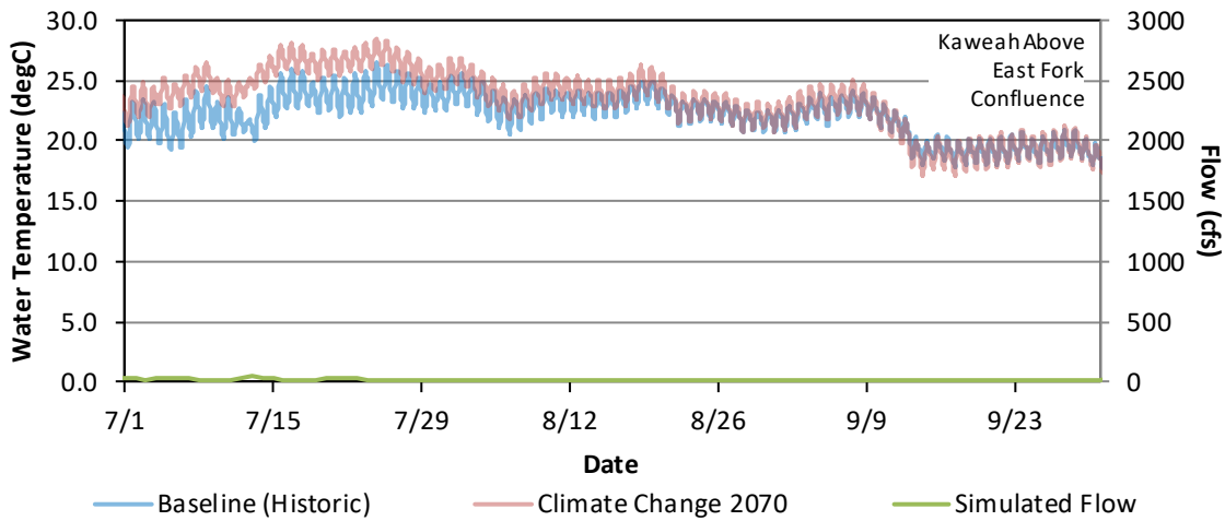
Figure G - 89. Hourly Water Temperature and Daily Average Flow Model Results for the Baseline (Historic) and Climate Change 2070 for Kaweah River Upstream of the Confluence with the East Fork, July 1 – September 30, 2018.
