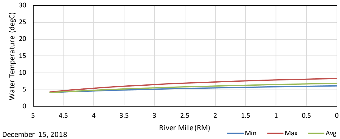
Figure F - 43. December 15, 2018 Unimpaired Maximum, Average, and Minimum Longitudinal Water Temperature Profiles in the East Fork of the Kaweah River Upstream of the Confluence with the Kaweah River.
