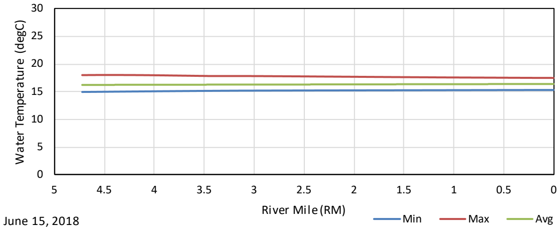
Figure F - 36. June 15, 2018 Baseline (Historic) Maximum, Average, and Minimum Longitudinal Water Temperature Profiles in the East Fork of the Kaweah River Upstream of the Confluence with the Kaweah River.
