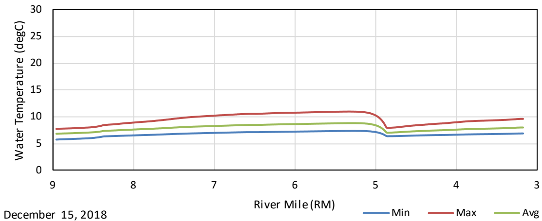
Figure G - 63. December 15, 2018 Climate Change 2030 Maximum, Average, and Minimum Longitudinal Water Temperature Profiles in the Kaweah River Upstream of the Confluence with the North Fork.
