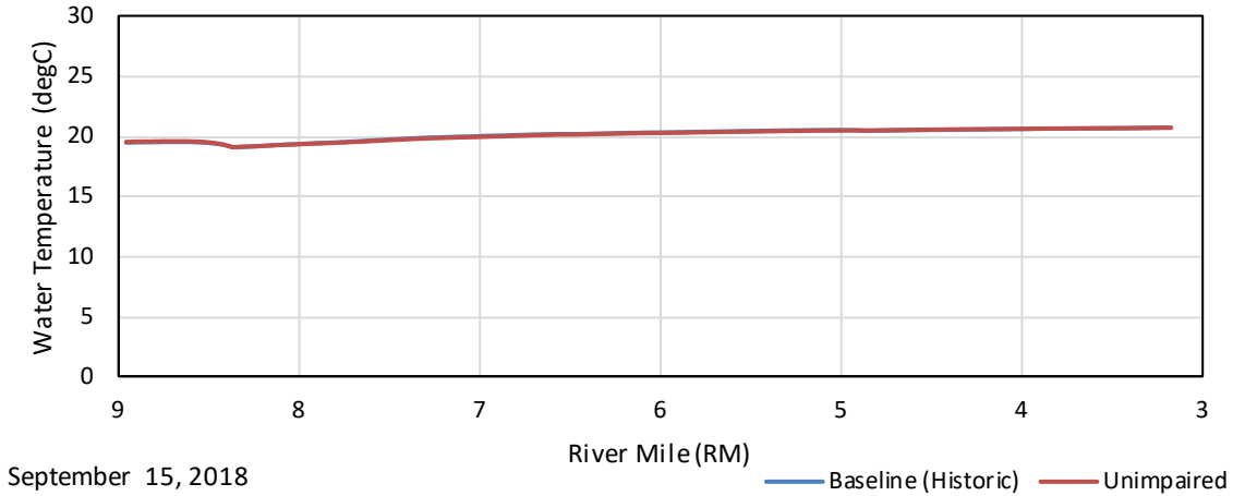
Figure F - 9. September 15, 2018 Average Longitudinal Water Temperature Profile in the Kaweah River from Upstream of the Confluence with the East Fork (RM8.95) to Upstream of the Confluence with the North Fork (RM3.17) for the Baseline (Historic) and Unimpaired Simulations.
