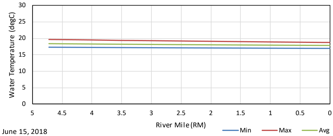
Figure G - 112. June 15, 2018 Climate Change 2070 Maximum, Average, and Minimum Longitudinal Water Temperature Profiles in the East Fork of the Kaweah River Upstream of the Confluence with the Mainstem.
