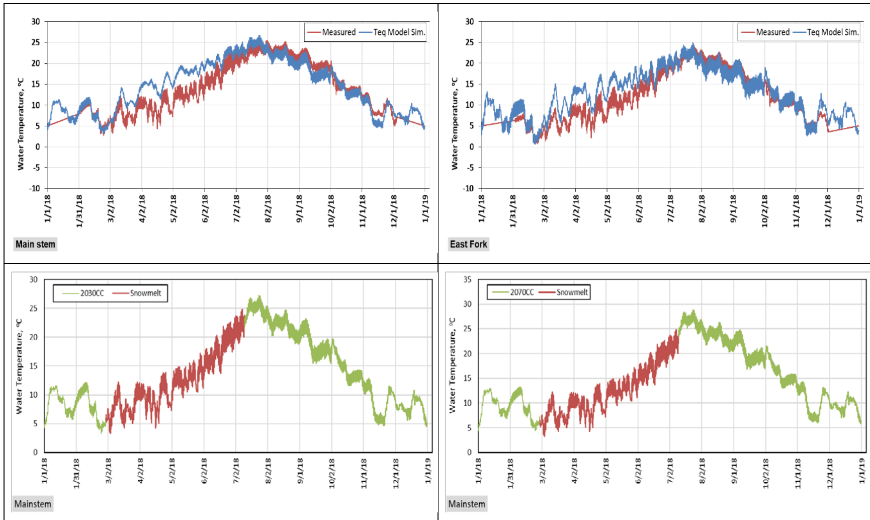
Figure AQ 4-9. Kaweah River at headwater: observed and estimated equilibrium water temperature: 2018 (Top left); East Fork Kaweah River at headwater: observed and estimated equilibrium water temperature: 2018. (Top Right); Calculated water headwater temperatures for the Kaweah River for 2030 climate conditions. (Bottom Left); Calculated water headwater temperatures for the Kaweah River for 2070 climate conditions. (Bottom Right)
