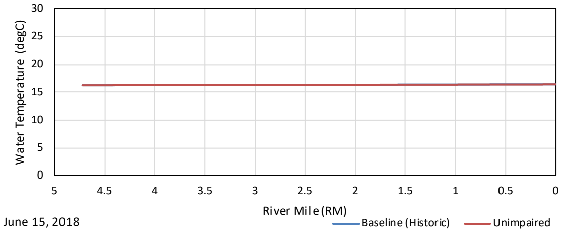
Figure F - 38. June 15, 2018 Average Longitudinal Water Temperature Profile in the East Fork of the Kaweah River Upstream of the Confluence with the Kaweah River for the Baseline (Historic) and Unimpaired Simulations.
