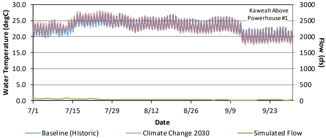
Figure G - 74. Hourly Water Temperature and Daily Average Flow Model Results for the Baseline (Historic) and Climate Change 2030 for Kaweah River Upstream of Powerhouse #1, July 1 – September 30, 2018.
