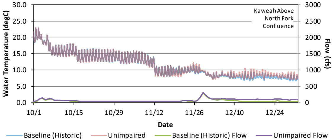
Figure F - 32. Hourly Water Temperature and Daily Average Flow Results for the Baseline (Historic) and Unimpaired Simulations for Kaweah River Upstream of the Confluence with the North Fork, October 1 – December 31, 2018.
