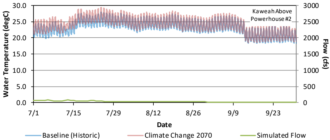
Figure G - 99. Hourly Water Temperature and Daily Average Flow Model Results for the Baseline (Historic) and Climate Change 2070 for Kaweah River Upstream of Powerhouse #2, July 1 – September 30, 2018.
