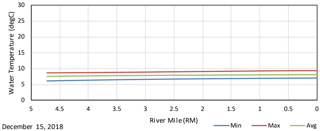
Figure G - 120. December 15, 2018 Climate Change 2070 Maximum, Average, and Minimum Longitudinal Water Temperature Profiles in the East Fork of the Kaweah River Upstream of the Confluence with the Mainstem.
