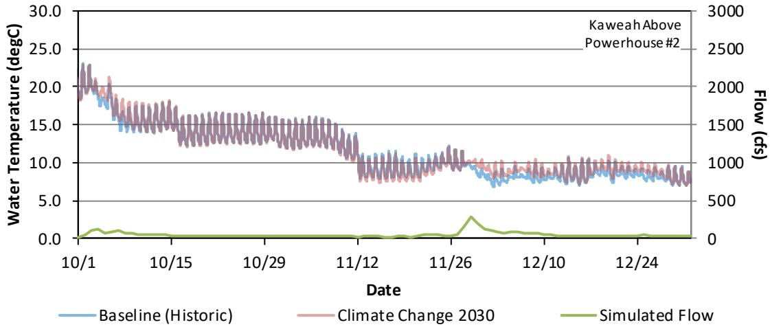
Figure G - 80. Hourly Water Temperature and Daily Average Flow Model Results for the Baseline (Historic) and Climate Change 2030 for Kaweah River Upstream of Powerhouse #2, October 1 – December 31, 2018.
