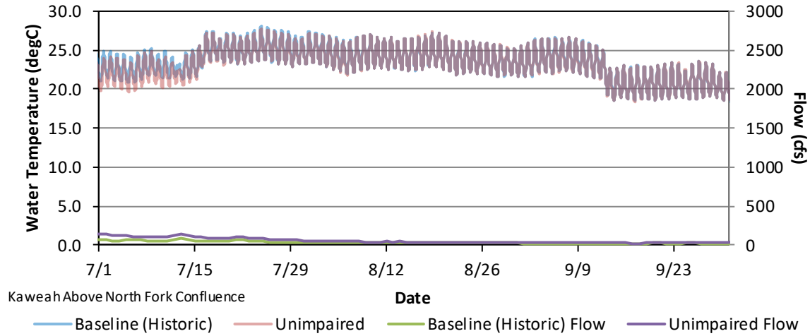
Figure F - 31. Hourly Water Temperature and Daily Average Flow Results for the Baseline (Historic) and Unimpaired Simulations for Kaweah River Upstream of the Confluence with the North Fork, July 1 – September 30, 2018.
