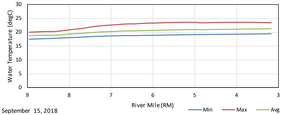
Figure G - 60. September 15, 2018 Climate Change 2070 Maximum, Average, and Minimum Longitudinal Water Temperature Profiles in the Kaweah River Upstream of Powerhouse #2.
