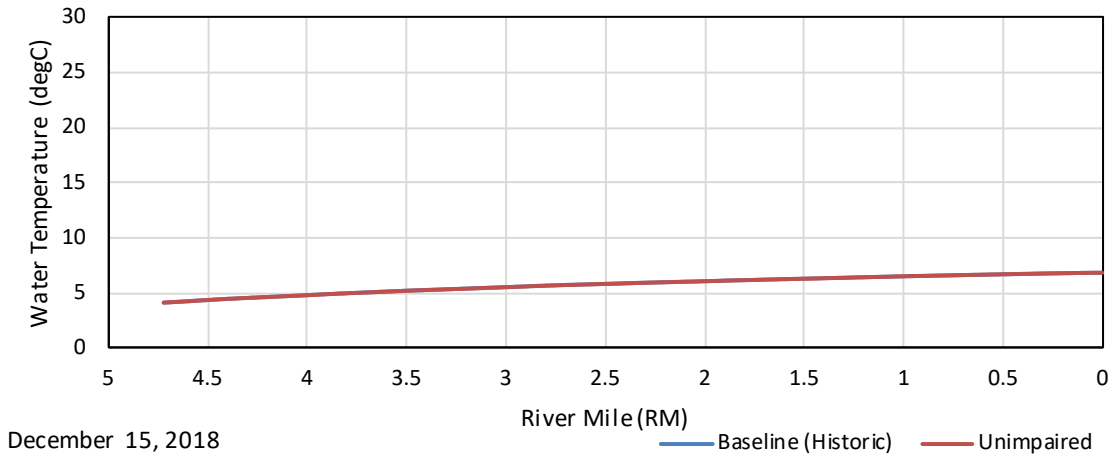
Figure F - 44. December 15, 2018 Average Longitudinal Water Temperature Profile in the East Fork of the Kaweah River Upstream of the Confluence with the for the Baseline (Historic) and Unimpaired Simulations.
