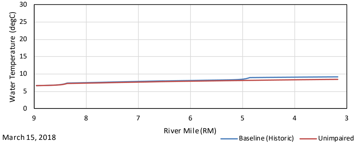
Figure F - 3. March 15, 2018 Average Longitudinal Water River Temperature Profile in the Kaweah River Upstream of the Confluence with the East Fork (RM8.95) to Upstream of the Confluence with the North Fork (RM3.17) for the Baseline (Historic) and Unimpaired Simulations.
