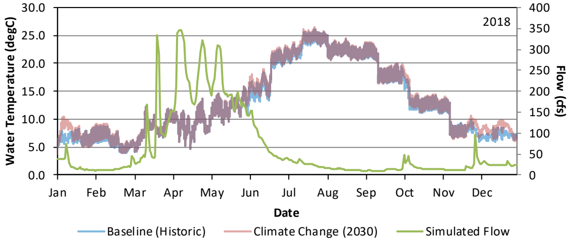
Figure AQ 4-12. Hourly Water Temperature Model Results Baseline (Existing) and Climate Change 2030 for East Fork of the Kaweah River Upstream of the Confluence with the Kaweah River for January 1 – December 31, 2018.
