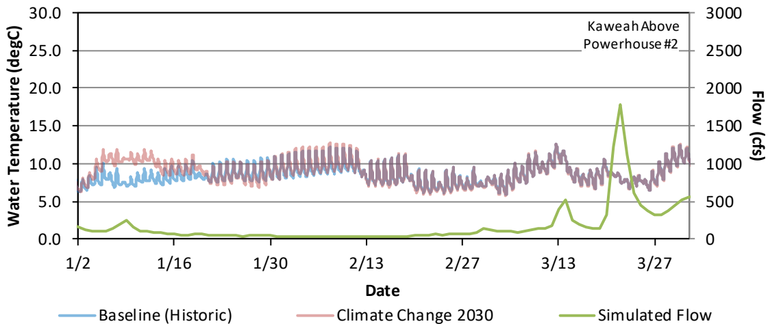
Figure G - 77. Hourly Water Temperature and Daily Average Flow Model Results for the Baseline (Historic) and Climate Change 2030 for Kaweah River Upstream of Powerhouse #2, January 1 – March 31, 2018.
