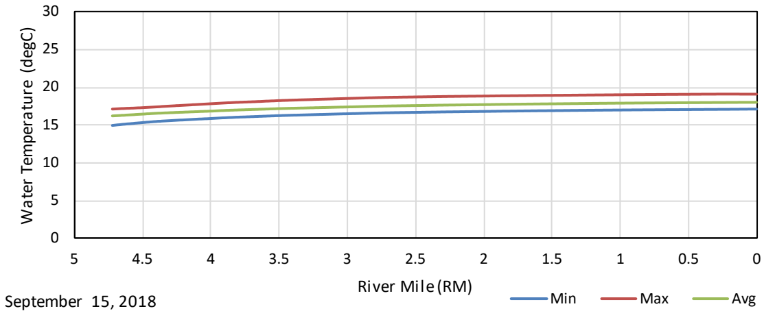
Figure F - 40. September 15, 2018 Unimpaired Maximum, Average, and Minimum Longitudinal Water Temperature Profiles in the East Fork of the Kaweah River Upstream of the Confluence with the Kaweah River.
