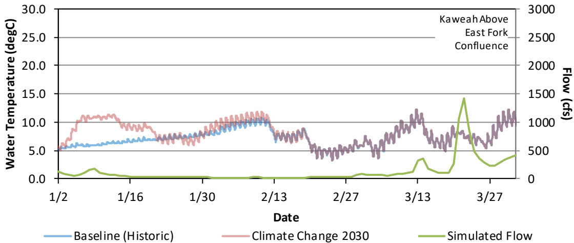
Figure G - 67. Hourly Water Temperature and Daily Average Flow Model Results for the Baseline (Historic) and Climate Change 2030 for Kaweah River Upstream of the Confluence with the East Fork, January 1 – March 31, 2018.
