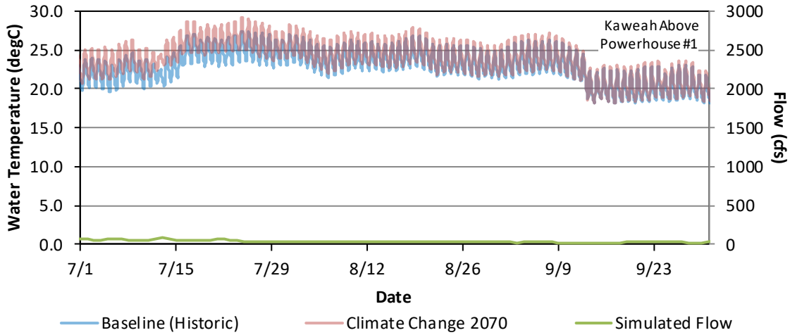
Figure G - 94. Hourly Water Temperature and Daily Average Flow Model Results for the Baseline (Historic) and Climate Change 2070 for Kaweah River Upstream of Powerhouse #1, July 1 – September 30, 2018.
