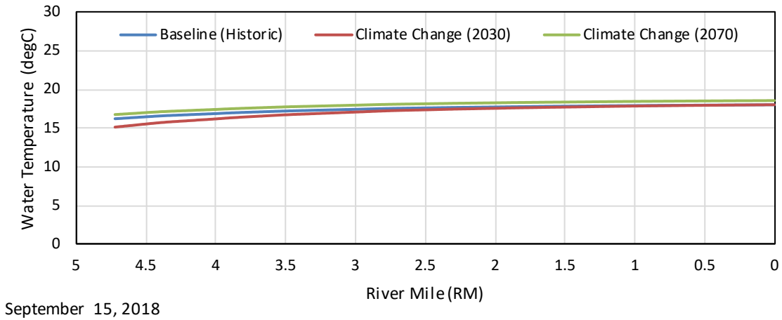
Figure G - 117. September 15, 2018 Average Longitudinal Water Temperature Profile in the East Fork of the Kaweah River Upstream of the Confluence with the Mainstem.
