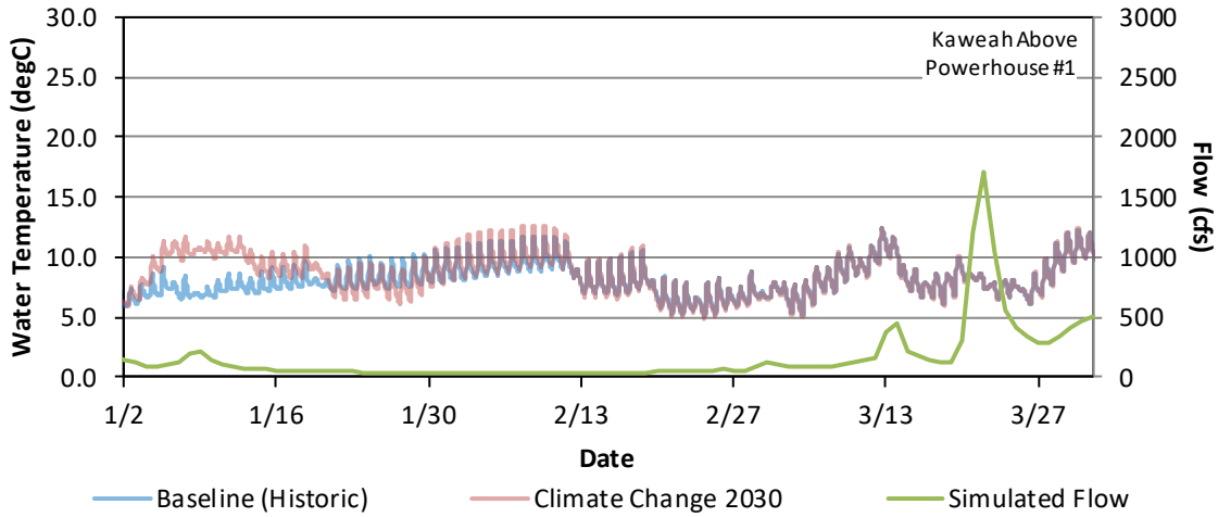
Figure G - 72. Hourly Water Temperature and Daily Average Flow Model Results for the Baseline (Historic) and Climate Change 2030 for Kaweah River Upstream of Powerhouse #1, January 1 – March 31, 2018.
