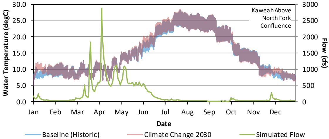
Figure AQ 4-10. Hourly Water Temperature and Daily Average Flow Model Results for the Baseline (Existing) and Climate Change 2030 for Kaweah River Upstream of the Confluence with the North Fork, January 1 – December 31, 2018.
