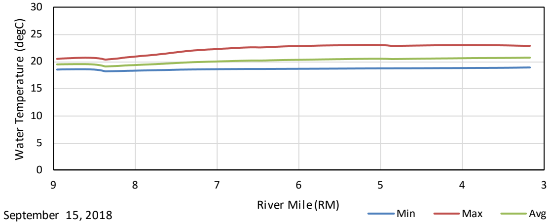
Figure F - 7. September 15, 2018 Baseline (Historic) Maximum, Average, and Minimum Longitudinal Water Temperature Profiles in the Kaweah River from Upstream of the Confluence with the East Fork (RM8.95) to Upstream of the Confluence with the North Fork (RM3.17).
