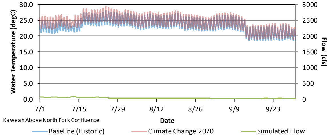
Figure G - 104. Hourly Water Temperature and Daily Average Flow Model Results for the Baseline (Historic) and Climate Change 2070 for Kaweah River Upstream of the Confluence with the North Fork, July 1 – September 30, 2018.
