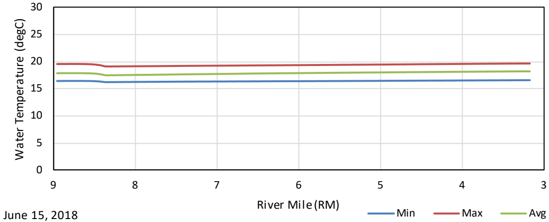
Figure F - 5. June 15, 2018 Unimpaired Maximum, Average, and Minimum Longitudinal Water Temperature Profiles in the Kaweah River from Upstream of the Confluence with the East Fork (RM8.95) to Upstream of the Confluence with the North Fork (RM3.17).
