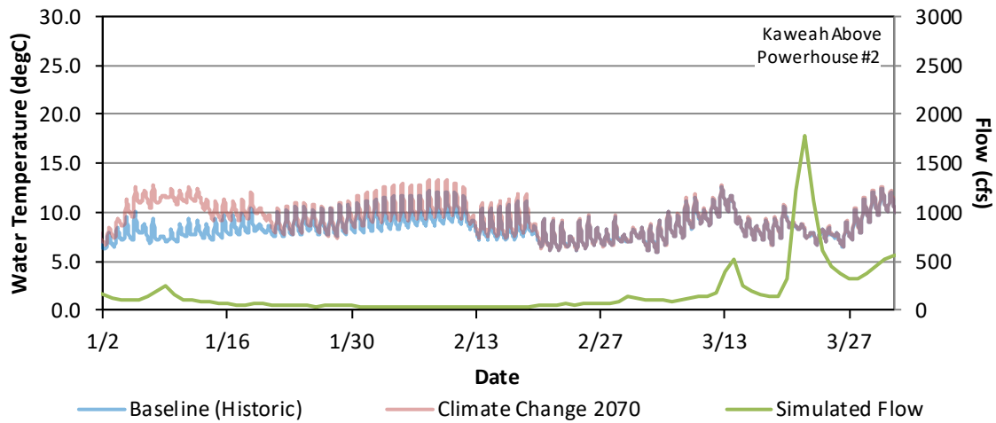
Figure G - 97. Hourly Water Temperature and Daily Average Flow Model Results for the Baseline (Historic) and Climate Change 2070 for Kaweah River Upstream of Powerhouse #2, January 1 – March 31, 2018.
