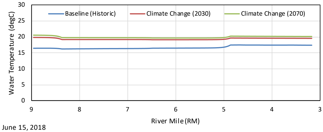
Figure G - 57. June 15, 2018 Average Longitudinal Water Temperature Profile in the Kaweah River Upstream of Powerhouse #1.
