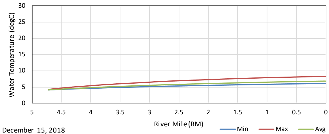
Figure F - 42. December 15, 2018 Baseline (Historic) Maximum, Average, and Minimum Longitudinal Water Temperature Profiles in the East Fork of the Kaweah River Upstream of the Confluence with the Kaweah River.
