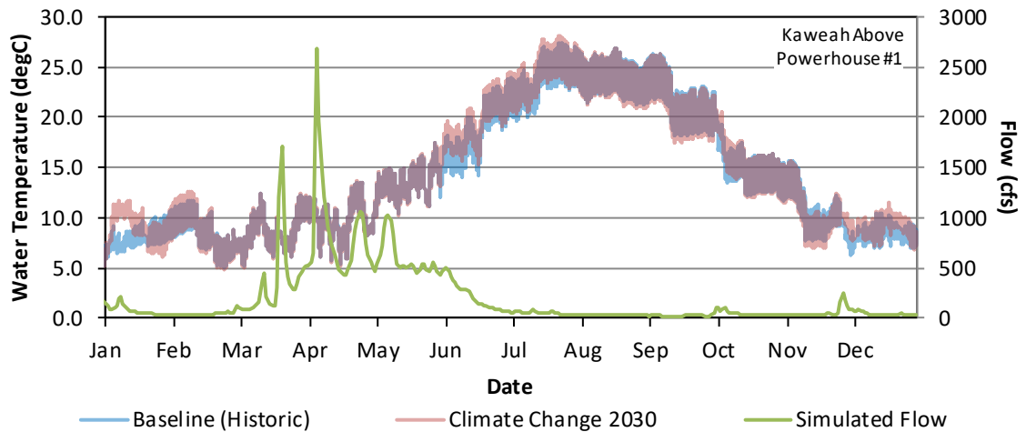
Figure G - 71. Hourly Water Temperature and Daily Average Flow Model Results for the Baseline (Historic) and Climate Change 2030 for Kaweah River Upstream of Powerhouse #1, January 1 – December 31, 2018.
