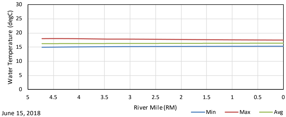
Figure G - 110. June 15, 2018 Baseline (Historic) Maximum, Average, and Minimum Longitudinal Water Temperature Profiles in the East Fork of the Kaweah River Upstream of the Confluence with the Mainstem.
