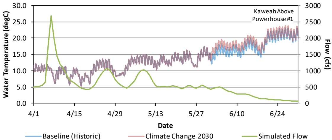
Figure G - 73. Hourly Water Temperature and Daily Average Flow Model Results for the Baseline (Historic) and Climate Change 2030 for Kaweah River Upstream of Powerhouse #1, April 1 – June 30, 2018.
