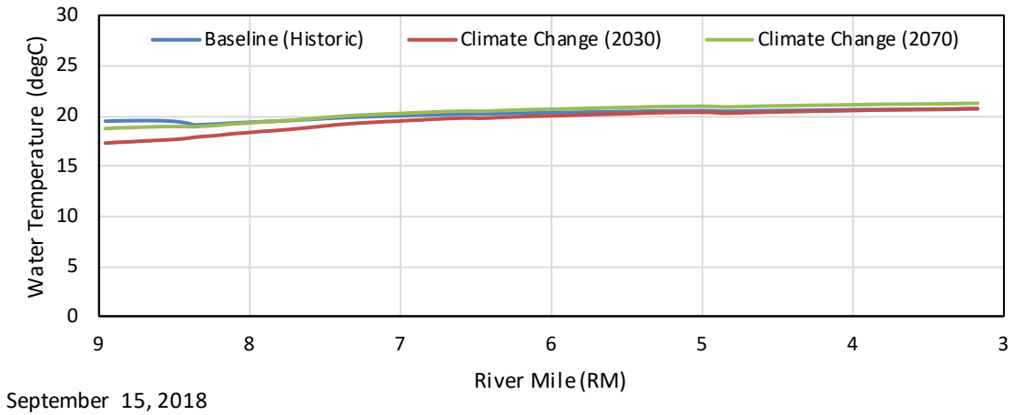
Figure G - 61. September 15, 2018 Average Longitudinal Water Temperature Profile in the Kaweah River Upstream of Powerhouse #2.
