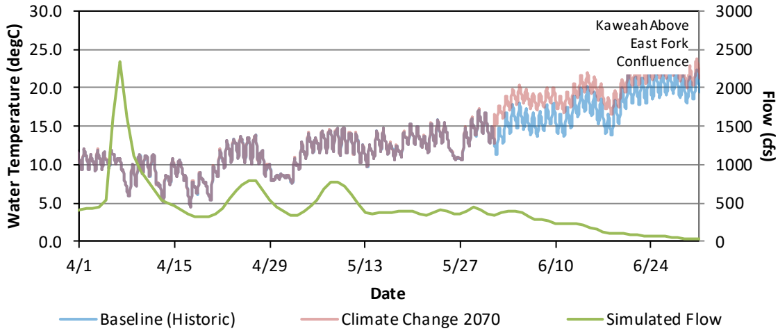
Figure G - 88. Hourly Water Temperature and Daily Average Flow Model Results for the Baseline (Historic) and Climate Change 2070 for Kaweah River Upstream of the Confluence with the East Fork, April 1 – June 30, 2018.
