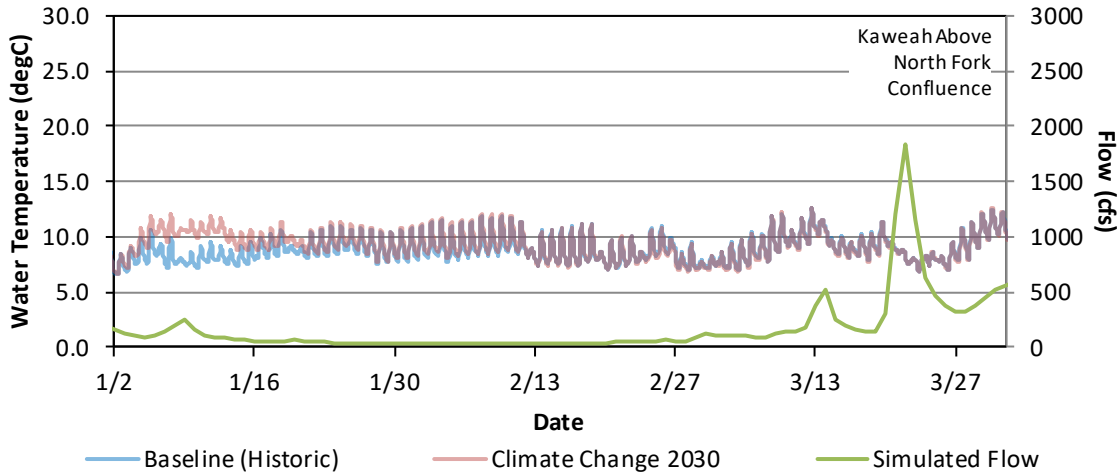
Figure G - 82. Hourly Water Temperature and Daily Average Flow Model Results for the Baseline (Historic) and Climate Change 2030 for Kaweah River Upstream of the Confluence with the North Fork, January 1 – March 31, 2018.
