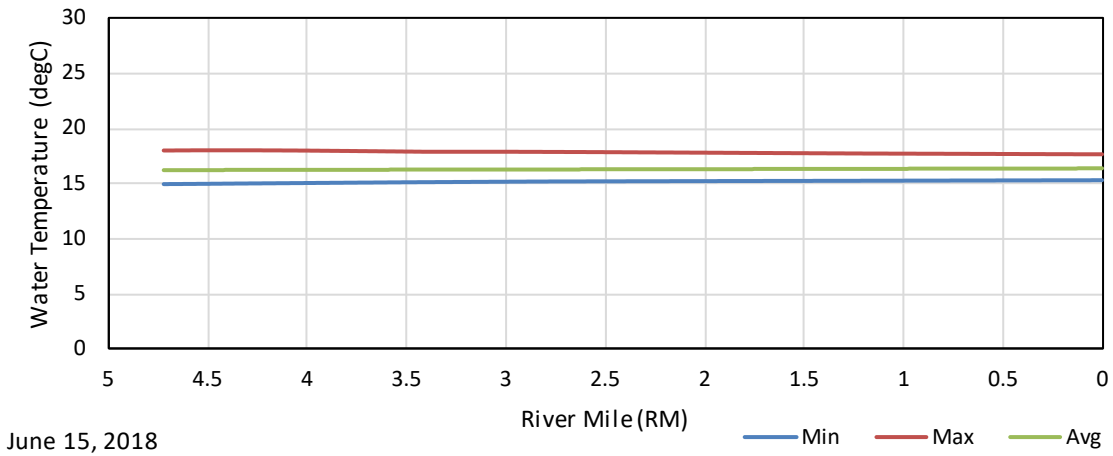
Figure F - 37. June 15, 2018 Unimpaired Maximum, Average, and Minimum Longitudinal Water Temperature Profiles in the East Fork of the Kaweah River Upstream of the Confluence with the Kaweah River.
