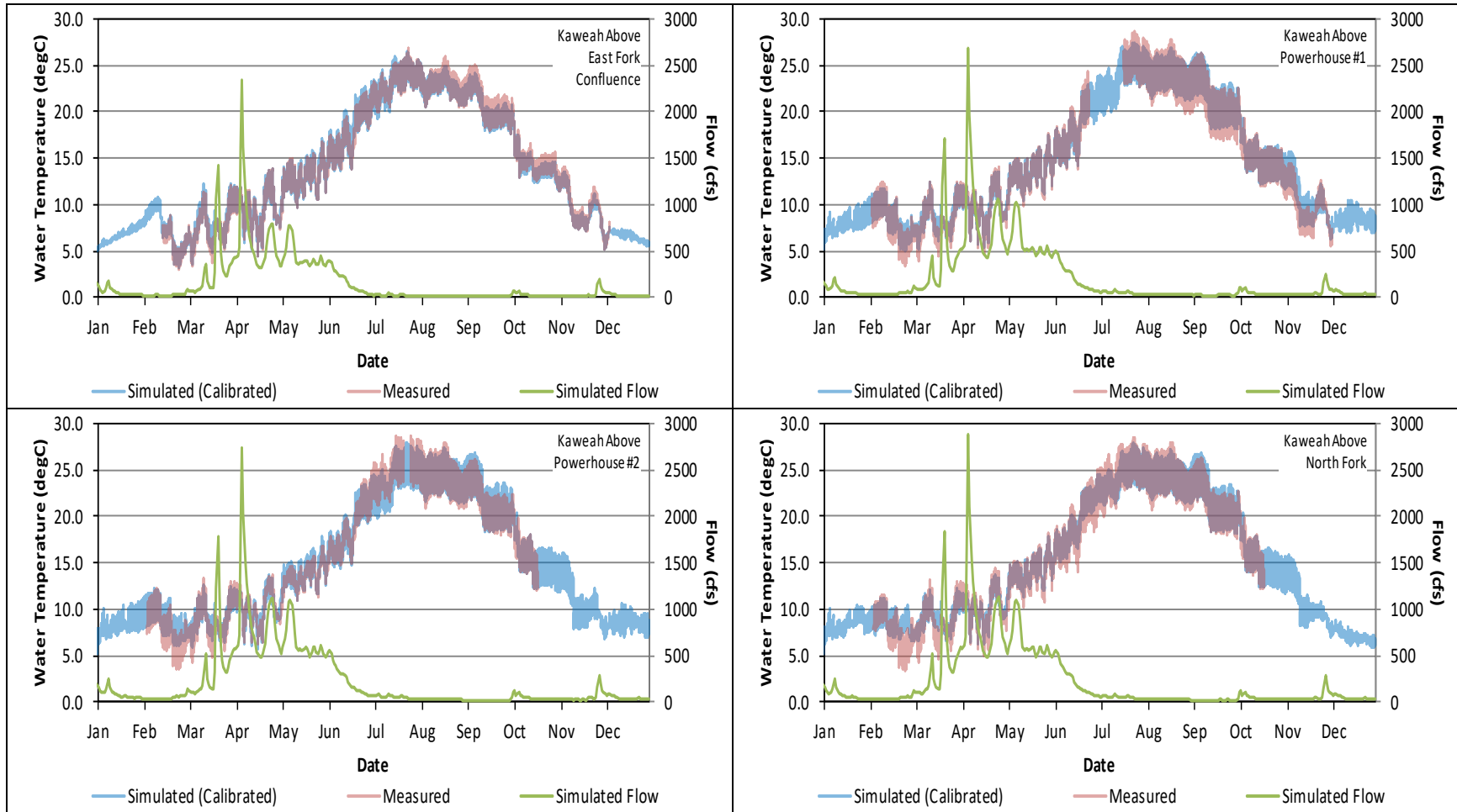
Figure AQ 4-3. Water Temperature Model Calibration Results for Kaweah River Upstream of the Confluence with the East Fork for January 1 – December 31, 2018.
