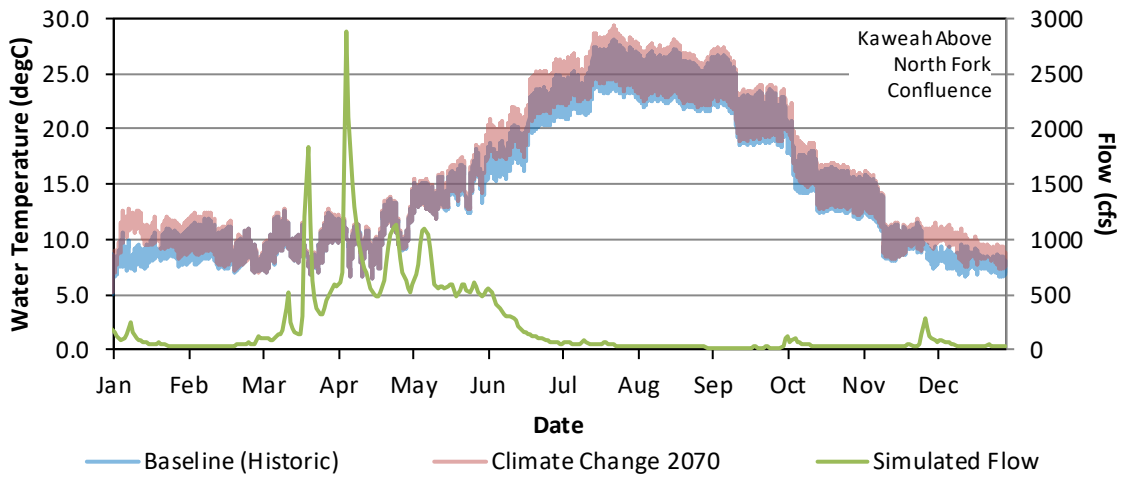
Figure G - 101. Hourly Water Temperature and Daily Average Flow Model Results for the Baseline (Historic) and Climate Change 2070 for Kaweah River Upstream of the Confluence with the North Fork, January 1 – December 31, 2018.
