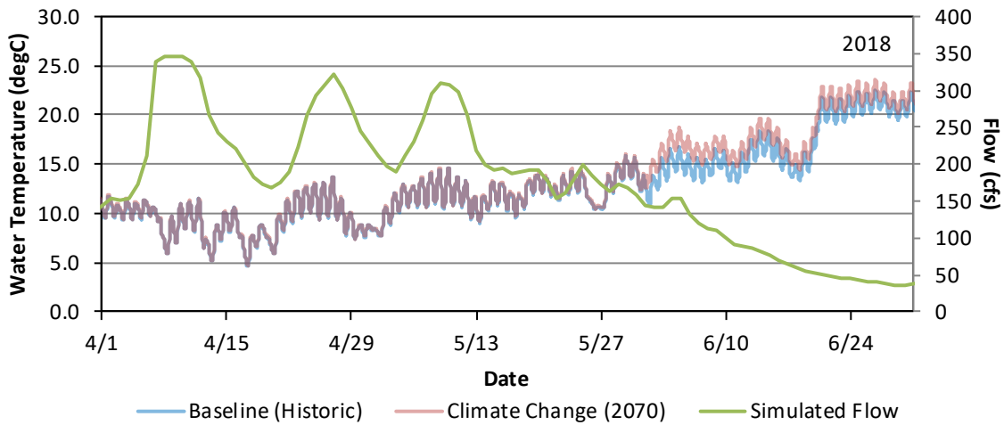
Figure G - 129. Hourly Water Temperature Model Results Baseline (Historic) and Climate Change 2070 for East Fork of the Kaweah River Upstream of the Confluence with the Kaweah River for April 1 – June 30, 2018.
