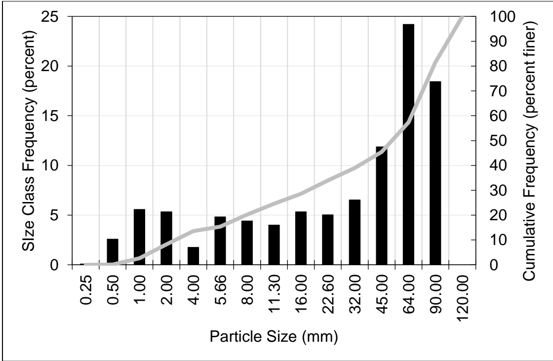
Figure B-17. East Fork Kaweah River Upstream of the Kaweah No. 1 Diversion: Histogram and Cumulative Particle Size Distribution, Sample 1 Subsample 1.
