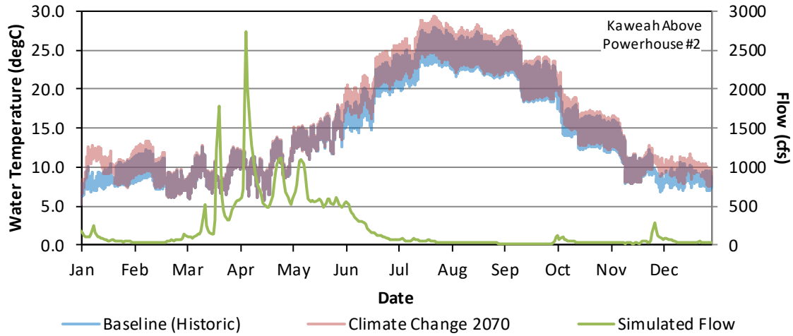
Figure G - 96. Hourly Water Temperature and Daily Average Flow Model Results for the Baseline (Historic) and Climate Change 2070 for Kaweah River Upstream of Powerhouse #2, January 1 – December 31, 2018.
