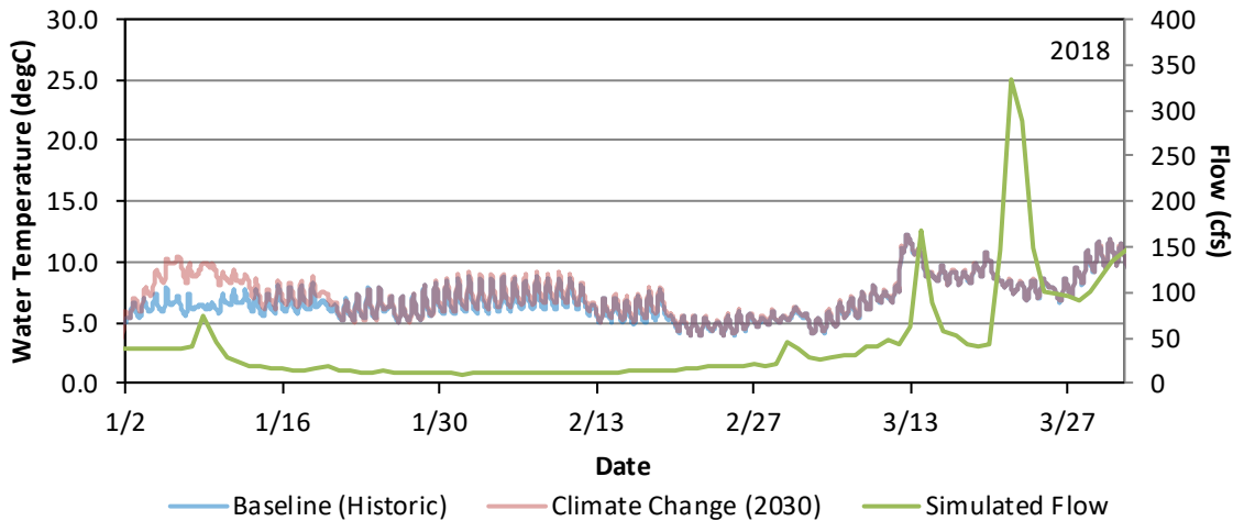
Figure G - 123. Hourly Water Temperature Model Results Baseline (Historic) and Climate Change 2030 East Fork of the Kaweah River Upstream of the Confluence with the Kaweah River for January 1 – March 31, 2018.
