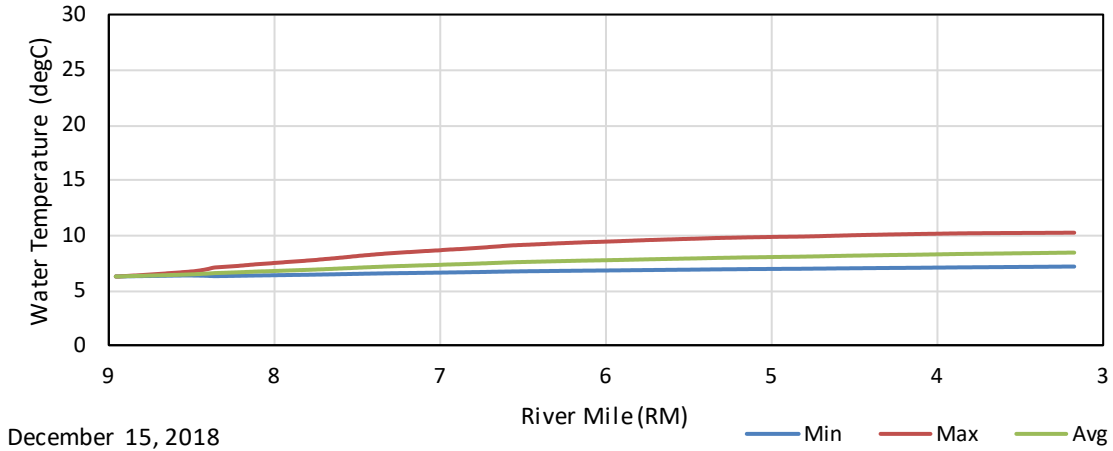
Figure F - 11. December 15, 2018 Unimpaired Maximum, Average, and Minimum Longitudinal Water Temperature Profiles in the Kaweah River from Upstream of the Confluence with the East Fork (RM8.95) to Upstream of the Confluence with the North Fork (RM3.17).
