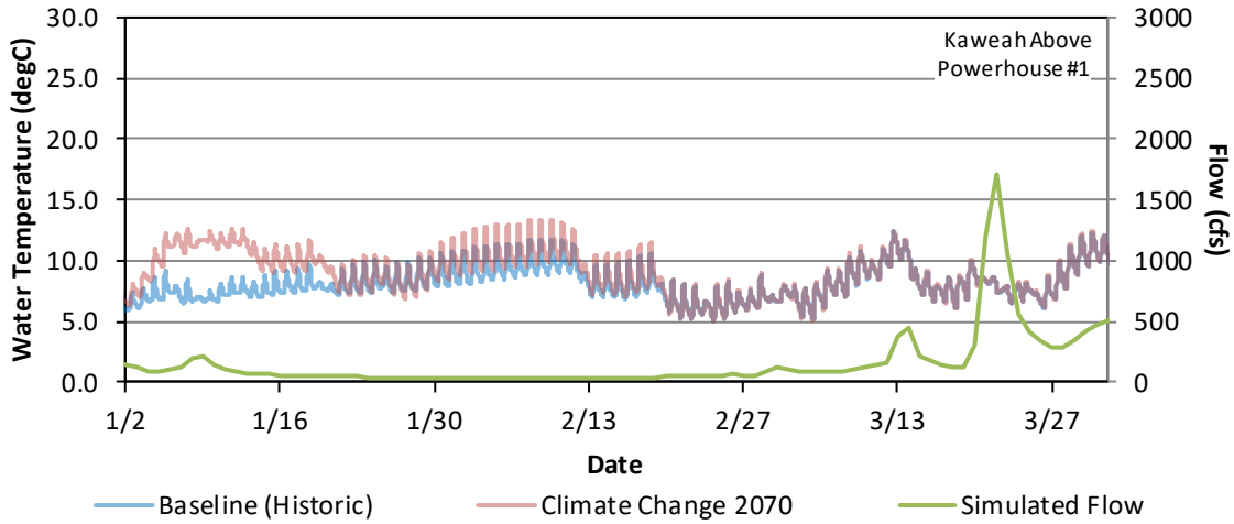
Figure G - 92. Hourly Water Temperature and Daily Average Flow Model Results for the Baseline (Historic) and Climate Change 2070 for Kaweah River Upstream of Powerhouse #1, January 1 – March 31, 2018.
