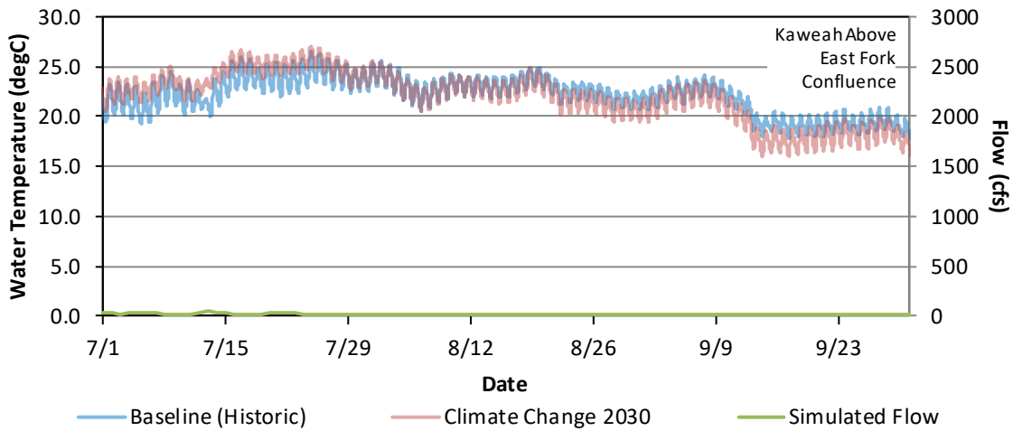
Figure G - 69. Hourly Water Temperature and Daily Average Flow Model Results for the Baseline (Historic) and Climate Change 2030 for Kaweah River Upstream of the Confluence with the East Fork, July 1 – September 30, 2018.
