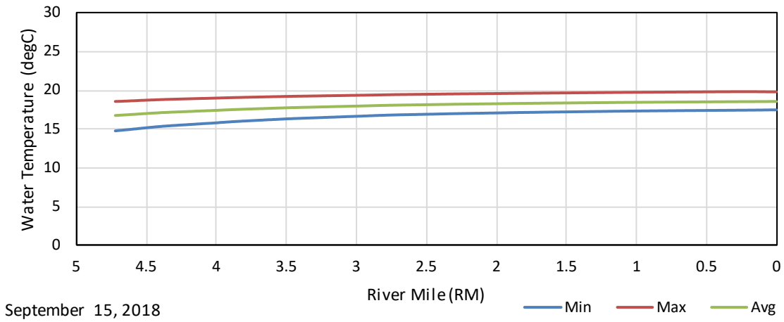
Figure G - 116. September 15, 2018 Climate Change 2070 Maximum, Average, and Minimum Longitudinal Water Temperature Profiles in the East Fork of the Kaweah River Upstream of the Confluence with the Mainstem.
