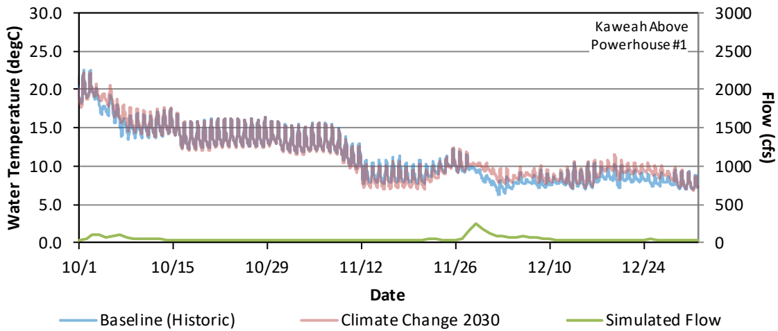
Figure G - 75. Hourly Water Temperature and Daily Average Flow Model Results for the Baseline (Historic) and Climate Change 2030 for Kaweah River Upstream of Powerhouse #1, October 1 – December 31, 2018.
