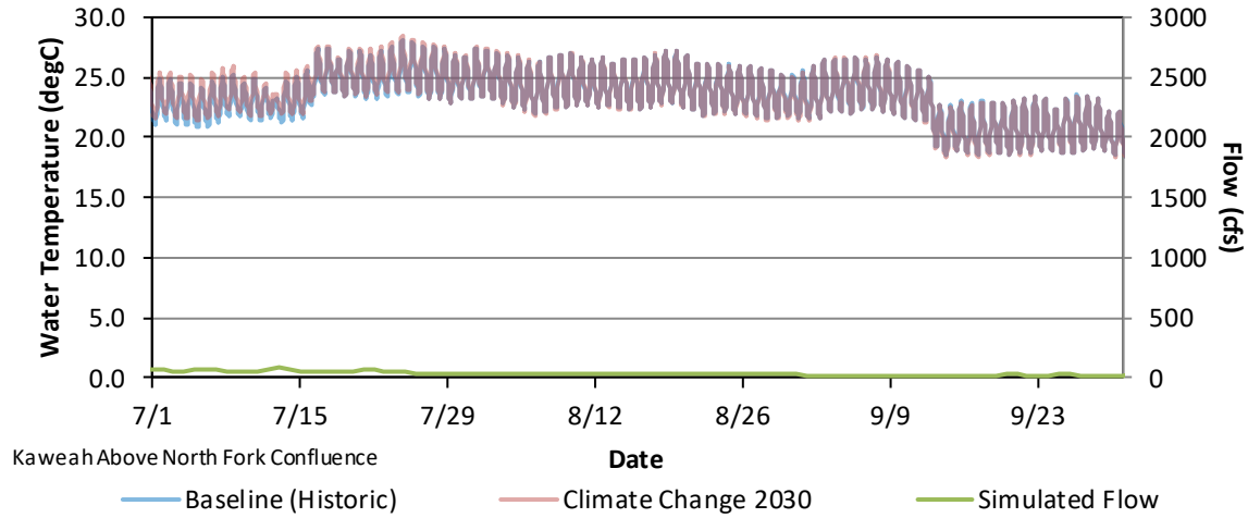
Figure G - 84. Hourly Water Temperature and Daily Average Flow Model Results for the Baseline (Historic) and Climate Change 2030 for Kaweah River Upstream of the Confluence with the North Fork, July 1 – September 30, 2018.
