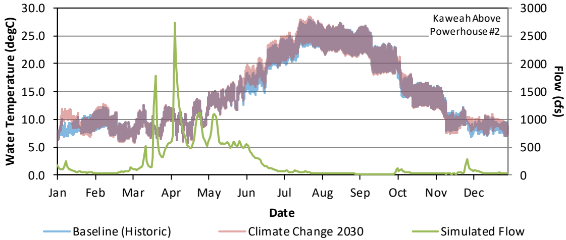
Figure G - 76. Hourly Water Temperature and Daily Average Flow Model Results for the Baseline (Historic) and Climate Change 2030 for Kaweah River Upstream of Powerhouse #2, January 1 – December 31, 2018.
