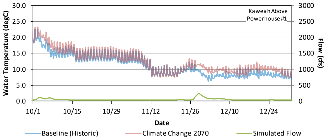
Figure G - 95. Hourly Water Temperature and Daily Average Flow Model Results for the Baseline (Historic) and Climate Change 2070 for Kaweah River Upstream of Powerhouse #1, October 1 – December 31, 2018.
