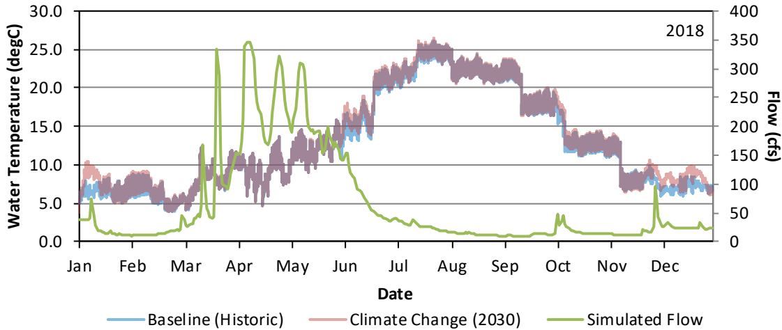
Figure G - 122. Hourly Water Temperature Model Results Baseline (Historic) and Climate Change 2030 for East Fork of the Kaweah River Upstream of the Confluence with the Kaweah River for January 1 – December 31, 2018.
