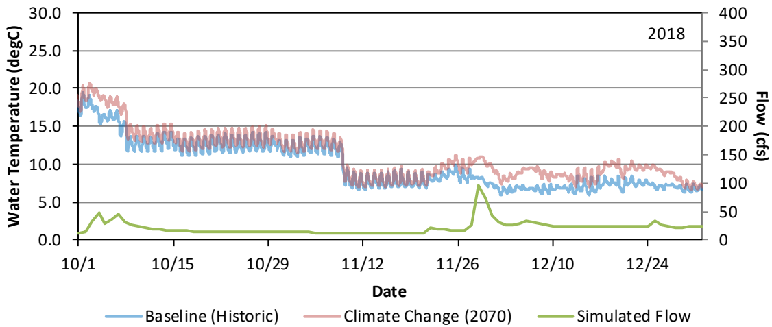
Figure G - 131. Hourly Water Temperature Model Results Baseline (Historic) and Climate Change 2070 for East Fork of the Kaweah River Upstream of the Confluence with the Kaweah River for October 1 – December 31, 2018.
