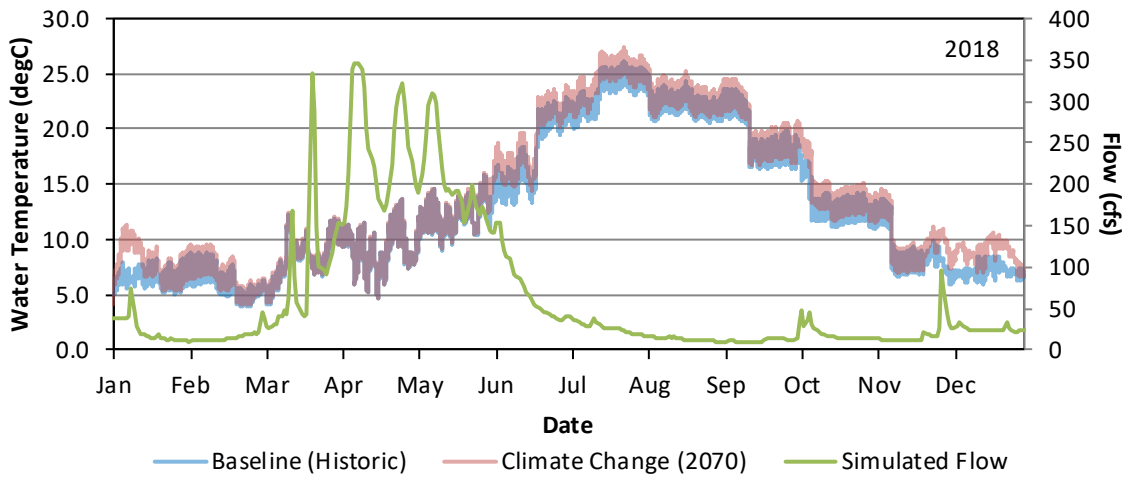
Figure G - 127. Hourly Water Temperature Model Results Baseline (Historic) and Climate Change 2070 for East Fork of the Kaweah River Upstream of the Confluence with the Kaweah River for January 1 – December 31, 2018.
