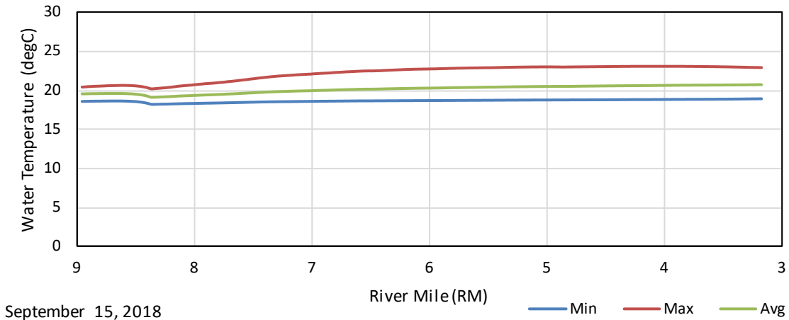
Figure F - 8. September 15, 2018 Unimpaired Maximum, Average, and Minimum Longitudinal Water Temperature Profiles in the Kaweah River from Upstream of the Confluence with the East Fork (RM8.95) to Upstream of the Confluence with the North Fork (RM3.17).
