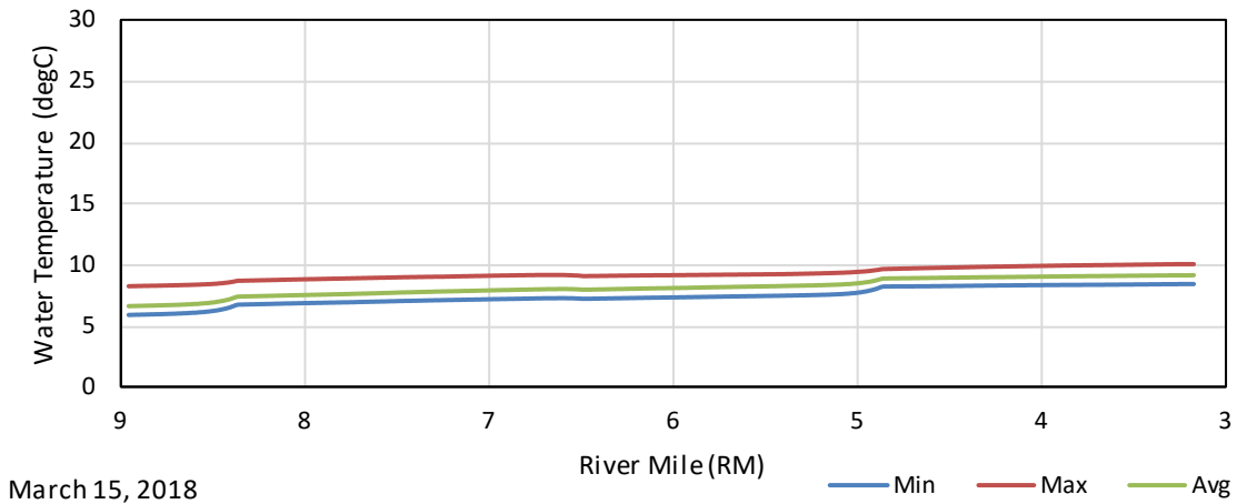
Figure G - 52. March 15, 2018 Climate Change 2070 Maximum, Average, and Minimum Longitudinal Water Temperature Profiles in the Kaweah River Upstream of the Confluence with the East Fork.
