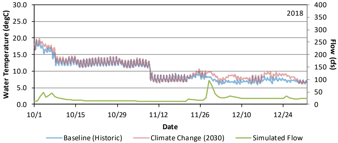
Figure G - 126. Hourly Water Temperature Model Results Baseline (Historic) and Climate Change 2030 for East Fork of the Kaweah River Upstream of the Confluence with the Kaweah River for October 1 – December 31, 2018.
