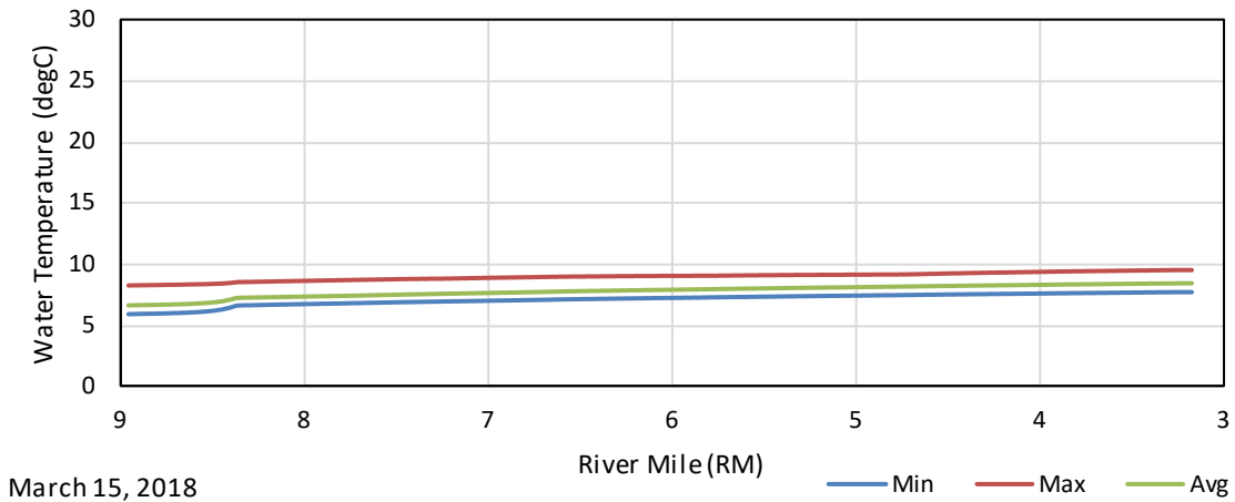
Figure F - 2. March 15, 2018 Unimpaired Maximum, Average, and Minimum Longitudinal Water Temperature Profiles in the Kaweah River from Upstream of the Confluence with the East Fork (RM8.95) to Upstream of the Confluence with the North Fork (RM3.17).
