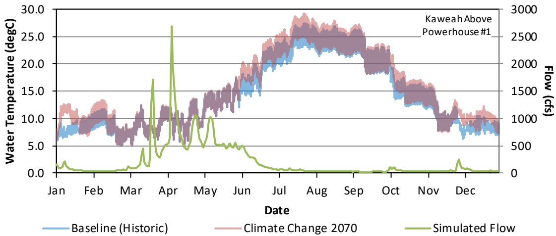
Figure G - 91. Hourly Water Temperature and Daily Average Flow Model Results for the Baseline (Historic) and Climate Change 2070 for Kaweah River Upstream of Powerhouse #1, January 1 – December 31, 2018.
