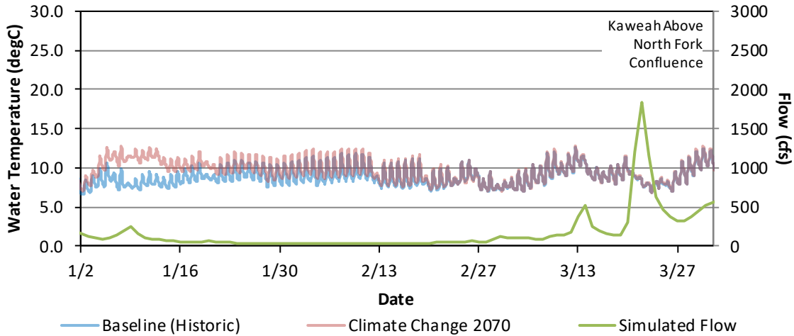
Figure G - 102. Hourly Water Temperature and Daily Average Flow Model Results for the Baseline (Historic) and Climate Change 2070 for Kaweah River Upstream of the Confluence with the North Fork, January 1 – March 31, 2018.
