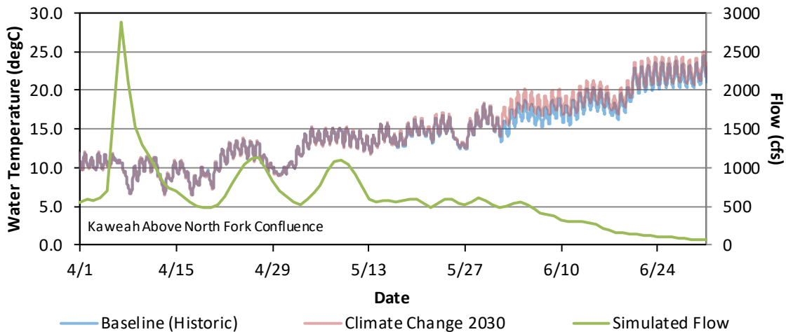
Figure G - 83. Hourly Water Temperature and Daily Average Flow Model Results for the Baseline (Historic) and Climate Change 2030 for Kaweah River Upstream of the Confluence with the North Fork, April 1 – June 30, 2018.
