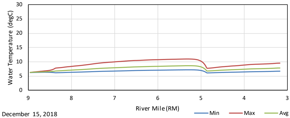
Figure G - 62. December 15, 2018 Baseline (Historic) Maximum, Average, and Minimum Longitudinal Water Temperature Profiles in the Kaweah River Upstream of the Confluence with the North Fork.
