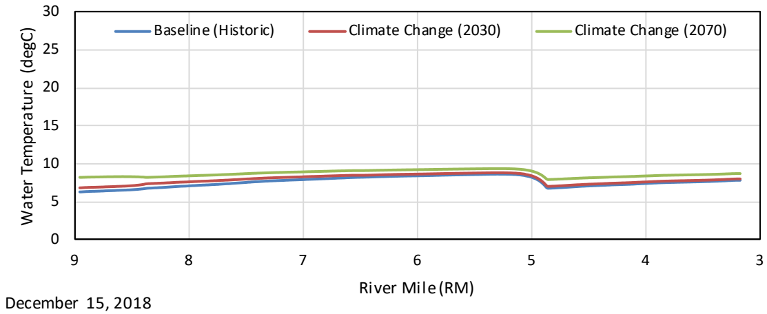
Figure G - 65. December 15, 2018 Average Longitudinal Water Temperature Profile in the Kaweah River Upstream of the Confluence with the North Fork.
