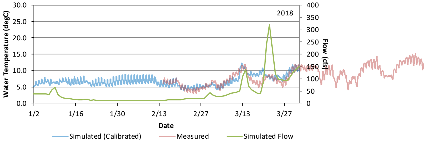
Figure E- 22. Water Temperature Model Calibration Results for East Fork of the Kaweah River Upstream of the Confluence with the Kaweah River for January 1 – March 31, 2018.
