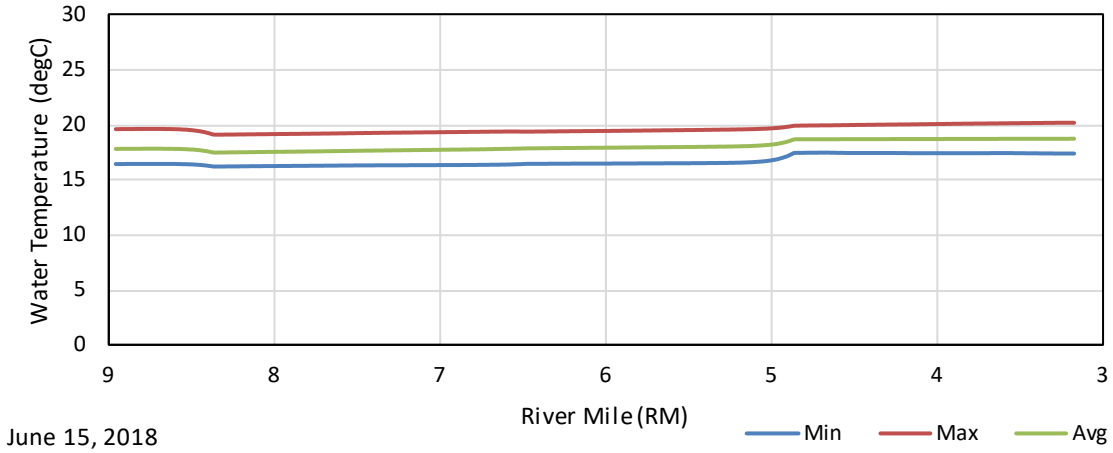
Figure G - 54. June 15, 2018 Baseline (Historic) Maximum, Average, and Minimum Longitudinal Water Temperature Profiles in the Kaweah River Upstream of Powerhouse #1.
