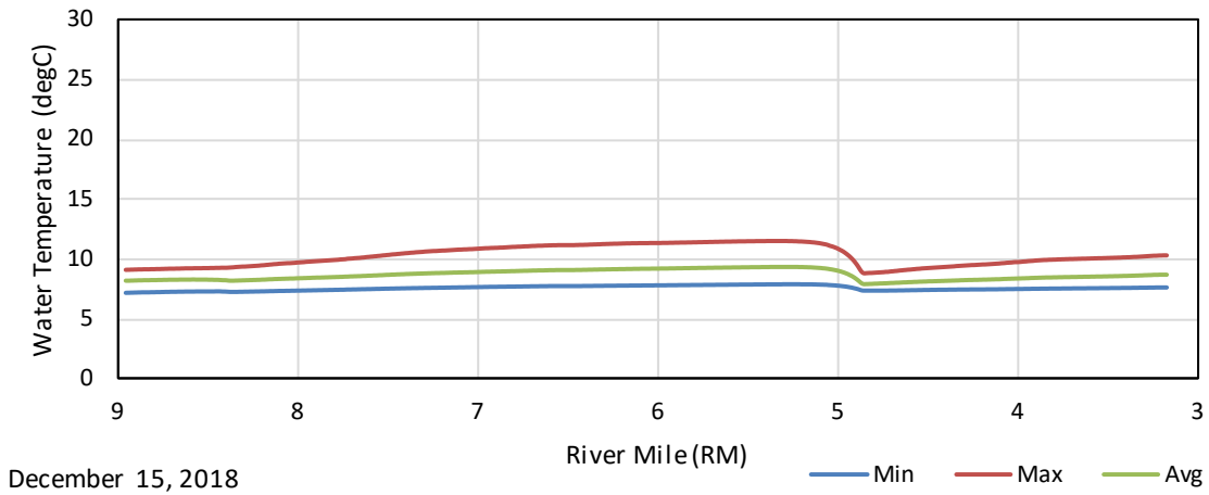
Figure G - 64. December 15, 2018 Climate Change 2070 Maximum, Average, and Minimum Longitudinal Water Temperature Profiles in the Kaweah River Upstream of the Confluence with the North Fork.
