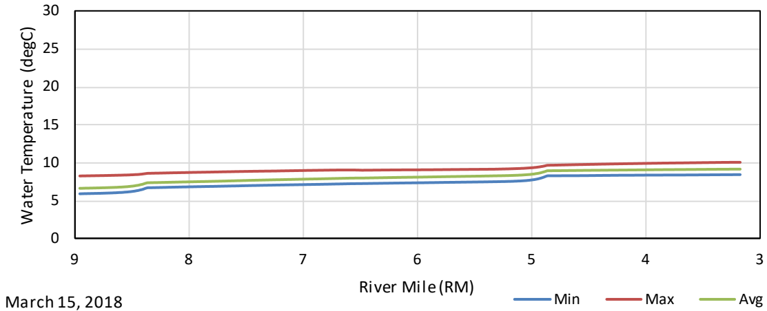
Figure G - 50. March 15, 2018 Baseline (Historic) Maximum, Average, and Minimum Longitudinal Water Temperature Profiles in the Kaweah River Upstream of the Confluence with the East Fork.
