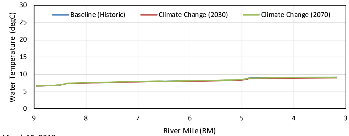
Figure G - 53. March 15, 2018 Average Longitudinal Water Temperature Profile in the Kaweah River Upstream of the Confluence with the East Fork.
