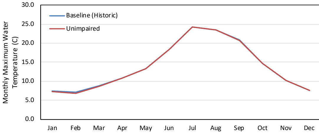
Figure AQ 4-8. Monthly Average Maximum Water Temperatures in the East Fork Kaweah River at the Confluence for the Baseline (Historic) and Unimpaired Flows
