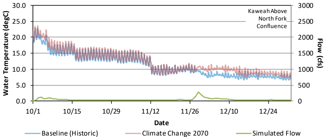
Figure G - 105. Hourly Water Temperature and Daily Average Flow Model Results for the Baseline (Historic) and Climate Change 2070 for Kaweah River Upstream of the Confluence with the North Fork, October 1 – December 31, 2018.
