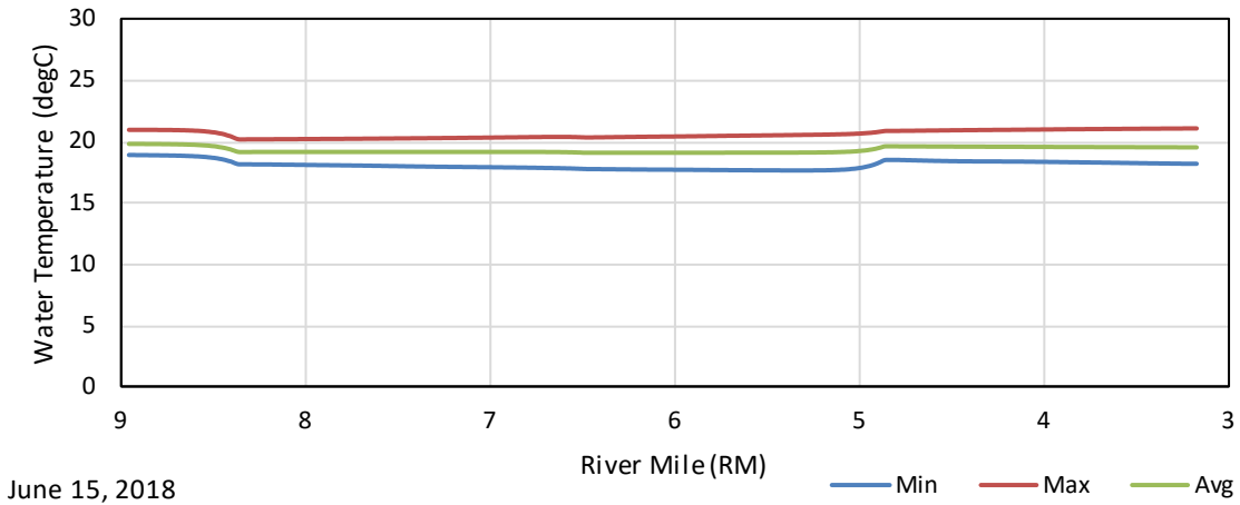
Figure G - 55. June 15, 2018 Climate Change 2030 Maximum, Average, and Minimum Longitudinal Water Temperature Profiles in the Kaweah River Upstream of Powerhouse #1.
