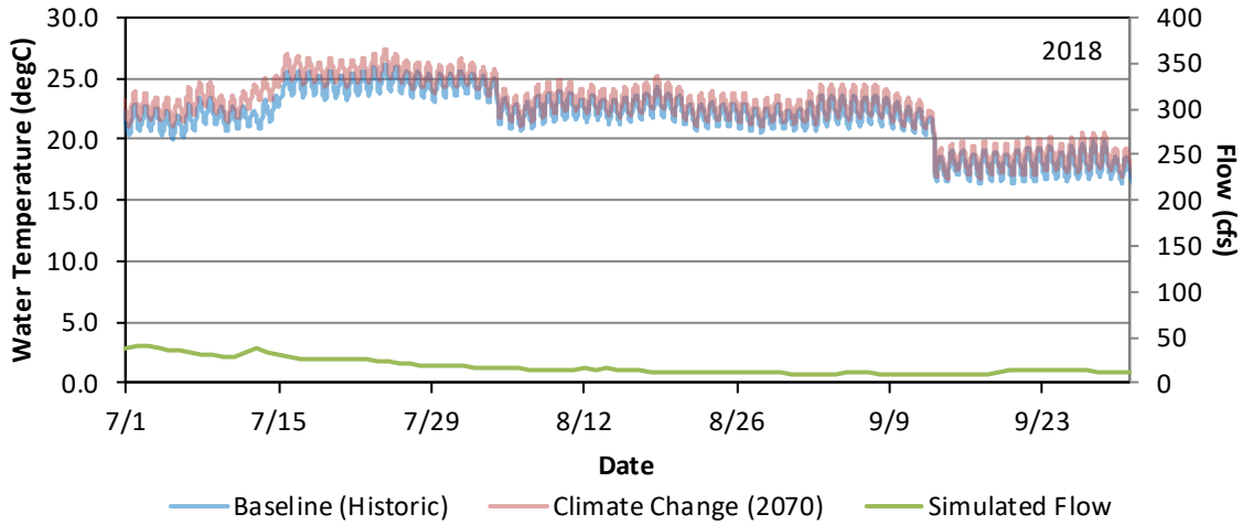
Figure G - 130. Hourly Water Temperature Model Results Baseline (Historic) and Climate Change 2070 for East Fork of the Kaweah River Upstream of the Confluence with the Kaweah River for July 1 – September 30, 2018.
