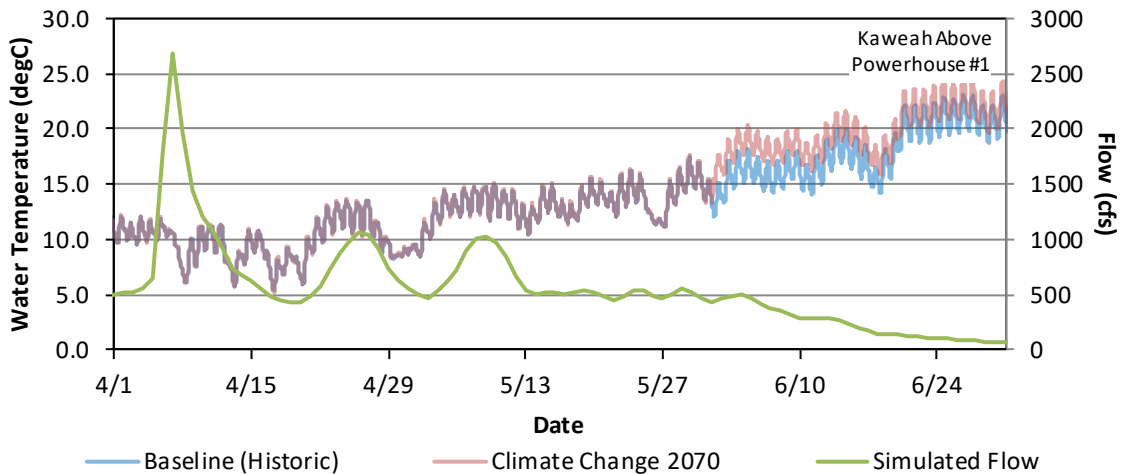
Figure G - 93. Hourly Water Temperature and Daily Average Flow Model Results for the Baseline (Historic) and Climate Change 2070 for Kaweah River Upstream of Powerhouse #1, April 1 – June 30, 2018.
