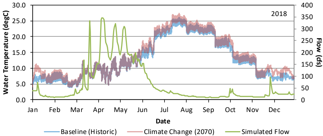
Figure AQ 4-13. Hourly Water Temperature Model Results Baseline (Historic) and Climate Change 2070 for East Fork of the Kaweah River Upstream of the Confluence with the Kaweah River for January 1 – December 31, 2018.
