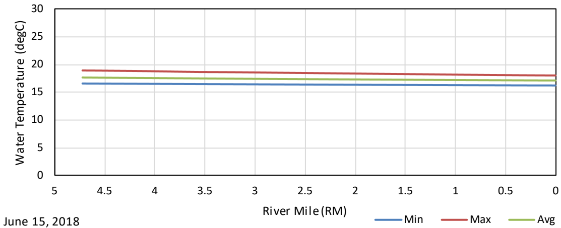
Figure G - 111. June 15, 2018 Climate Change 2030 Maximum, Average, and Minimum Longitudinal Water Temperature Profiles in the East Fork of the Kaweah River Upstream of the Confluence with the Mainstem.
