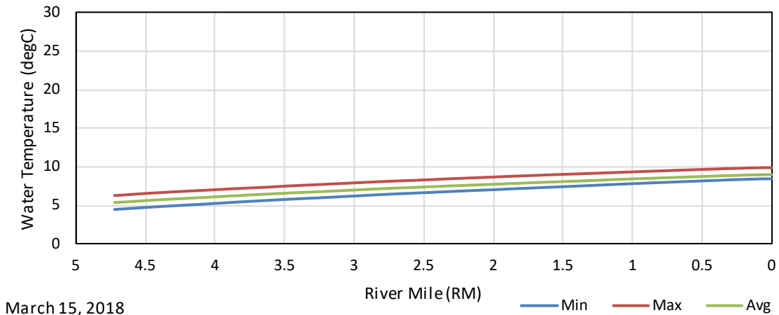
Figure G - 107. March 15, 2018 Climate Change 2030 Maximum, Average, and Minimum Longitudinal Water Temperature Profiles in the East Fork of the Kaweah River Upstream of the Confluence with the Mainstem.
