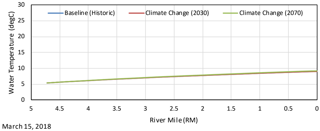
Figure G - 109. March 15, 2018 Average Longitudinal Water Temperature Profile in the East Fork of the Kaweah River Upstream of the Confluence with the Mainstem.
