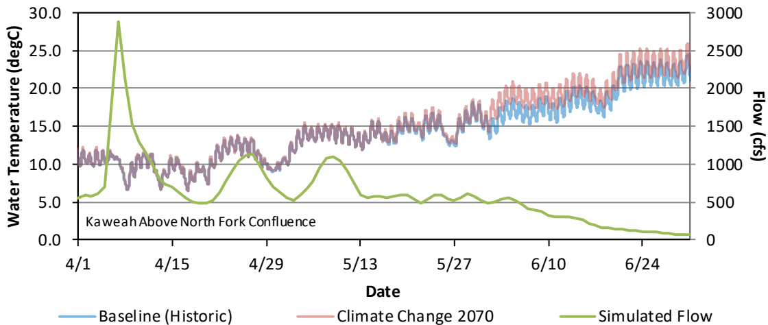
Figure G - 103. Hourly Water Temperature and Daily Average Flow Model Results for the Baseline (Historic) and Climate Change 2070 for Kaweah River Upstream of the Confluence with the North Fork, April 1 – June 30, 2018.
