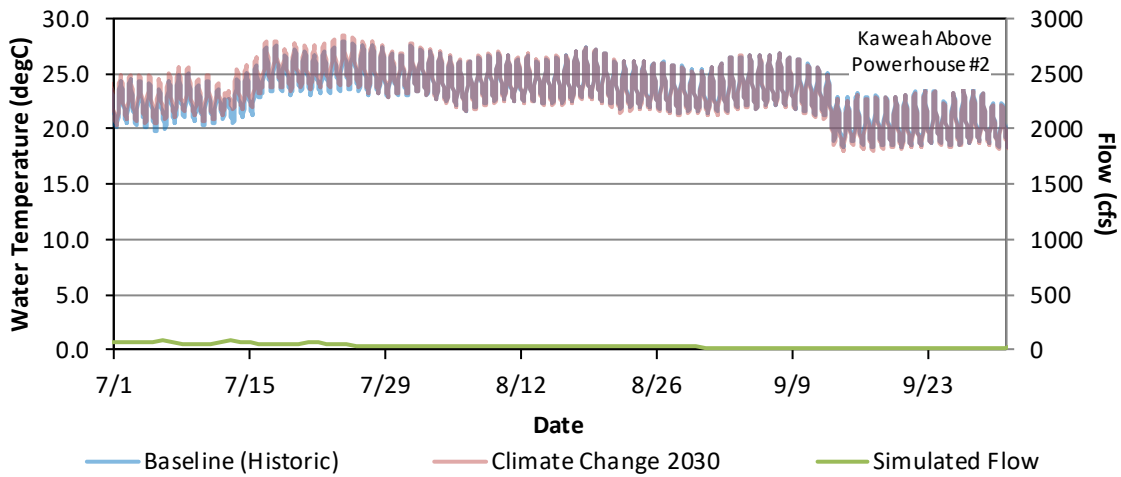
Figure G - 79. Hourly Water Temperature and Daily Average Flow Model Results for the Baseline (Historic) and Climate Change 2030 for Kaweah River Upstream of Powerhouse #2, July 1 – September 30, 2018.
