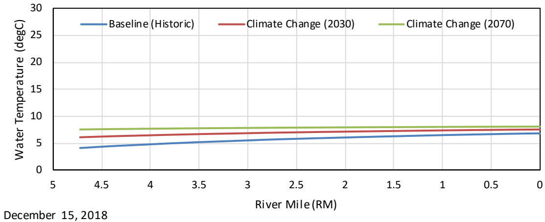
Figure G - 121. December 15, 2018 Average Longitudinal Water Temperature Profile in the East Fork of the Kaweah River Upstream of the Confluence with the Mainstem.
