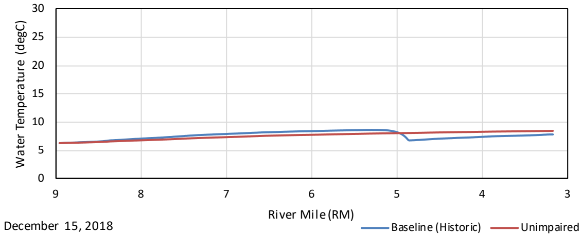
Figure F - 12. December 15, 2018 Average Longitudinal Water Temperature Profile in the Kaweah River from Upstream of the Confluence with the East Fork (RM8.95) to Upstream of the Confluence with the North Fork (RM3.17) for the Baseline (Historic) and Unimpaired Simulations.
