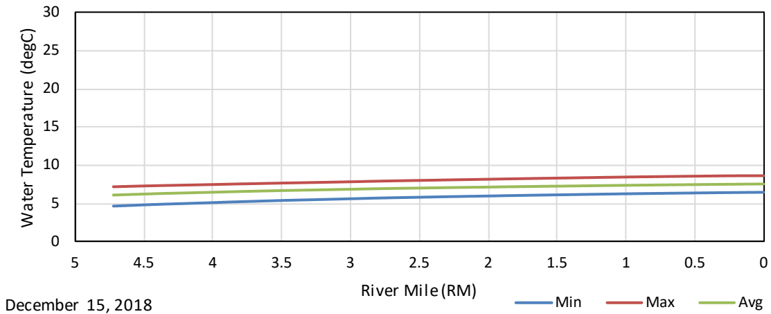
Figure G - 119. December 15, 2018 Climate Change 2030 Maximum, Average, and Minimum Longitudinal Water Temperature Profiles in the East Fork of the Kaweah River Upstream of the Confluence with the Mainstem.
