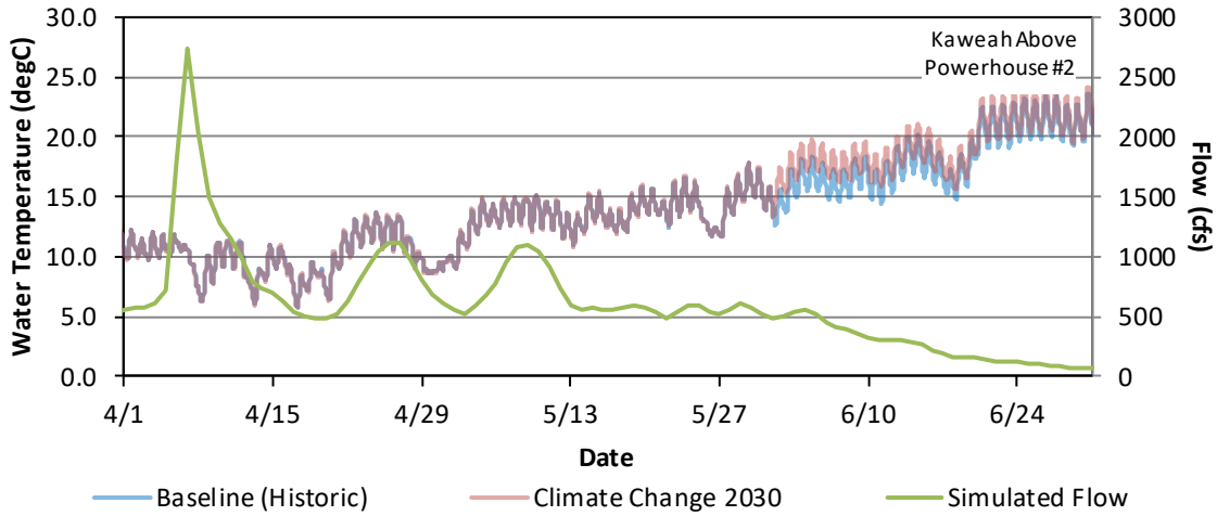
Figure G - 78. Hourly Water Temperature and Daily Average Flow Model Results for the Baseline (Historic) and Climate Change 2030 for Kaweah River Upstream of Powerhouse #2, April 1 – June 30, 2018.
