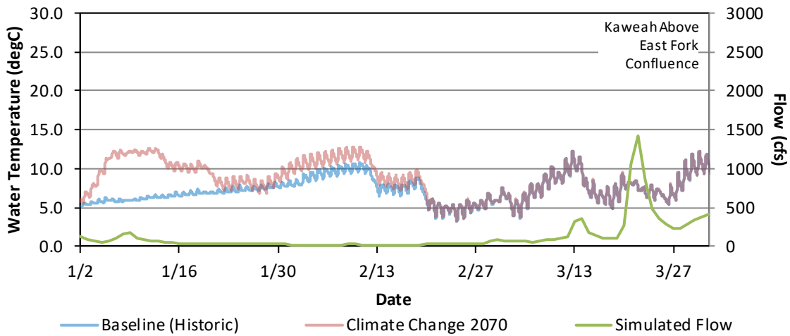
Figure G - 87. Hourly Water Temperature and Daily Average Flow Model Results for the Baseline (Historic) and Climate Change 2070 for Kaweah River Upstream of the Confluence with the East Fork, January 1 – March 31, 2018.
