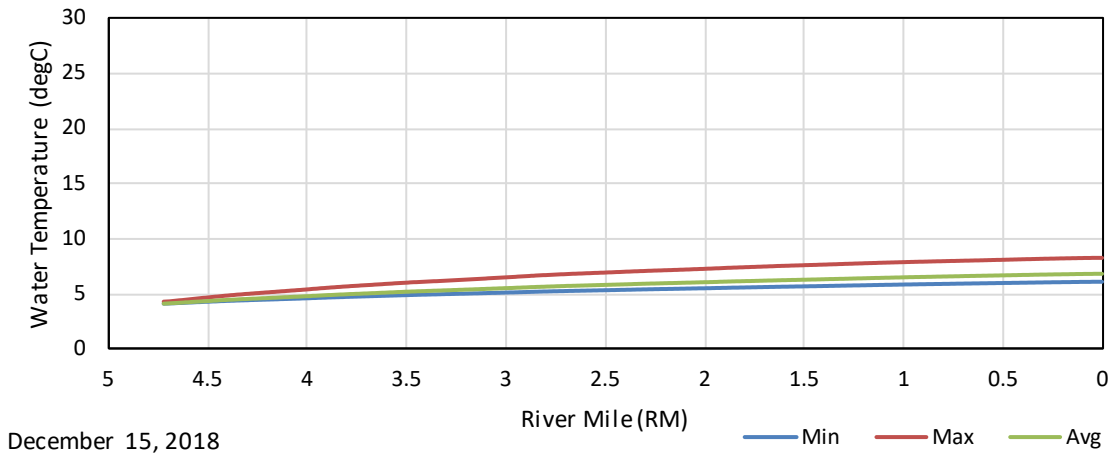
Figure G - 118. December 15, 2018 Baseline (Historic) Maximum, Average, and Minimum Longitudinal Water Temperature Profiles in the East Fork of the Kaweah River Upstream of the Confluence with the Mainstem.
