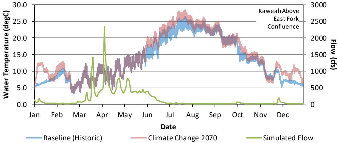
Figure G - 86. Hourly Water Temperature and Daily Average Flow Model Results for the Baseline (Historic) and Climate Change 2070 for Kaweah River Upstream of the Confluence with the East Fork, January 1 – December 31, 2018.
