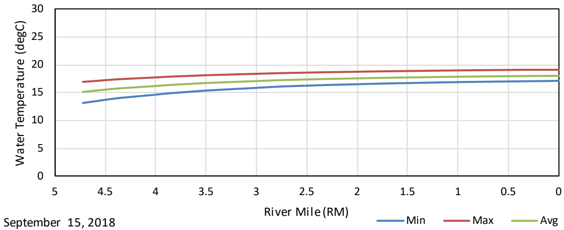
Figure G - 115. September 15, 2018 Climate Change 2030 Maximum, Average, and Minimum Longitudinal Water Temperature Profiles in the East Fork of the Kaweah River Upstream of the Confluence with the Mainstem.
