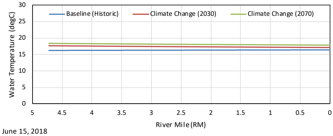
Figure G - 113. June 15, 2018 Average Longitudinal Water Temperature Profile in the East Fork of the Kaweah River Upstream of the Confluence with the Mainstem.
