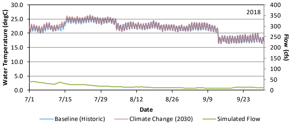
Figure G - 125. Hourly Water Temperature Model Results Baseline (Historic) and Climate Change 2030 for East Fork of the Kaweah River Upstream of the Confluence with the Kaweah River for July 1 – September 30, 2018.
