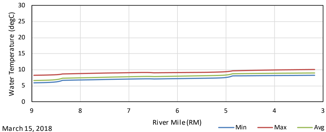
Figure G - 51. March 15, 2018 Climate Change 2030 Maximum, Average, and Minimum Longitudinal Water Temperature Profiles in the Kaweah River Upstream of the Confluence with the East Fork.
