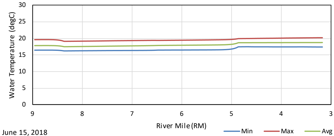
Figure F - 4. June 15, 2018 Baseline (Historic) Maximum, Average, and Minimum Longitudinal Water Temperature Profiles in the Kaweah River from Upstream of the Confluence with the East Fork (RM8.95) to Upstream of the Confluence with the North Fork (RM3.17).
