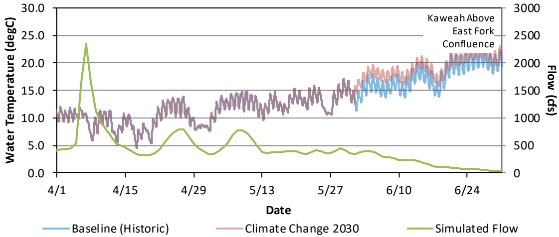
Figure G - 68. Hourly Water Temperature and Daily Average Flow Model Results for the Baseline (Historic) and Climate Change 2030 for Kaweah River Upstream of the Confluence with the East Fork, April 1 – June 30, 2018.
