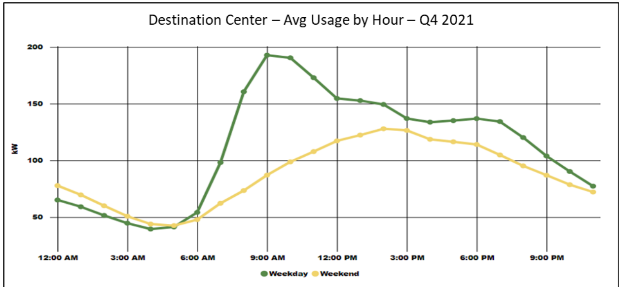
Figure 4.2 Destination Center Usage per Hour in Q4 2021: 33 sites/651 ports
