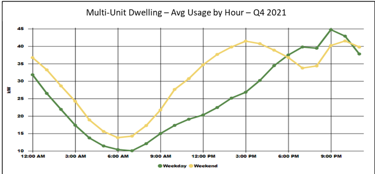
Figure 4.4 Multi-Unit Dwelling Usage per Hour in Q4 2021: 33 sites/383 ports
